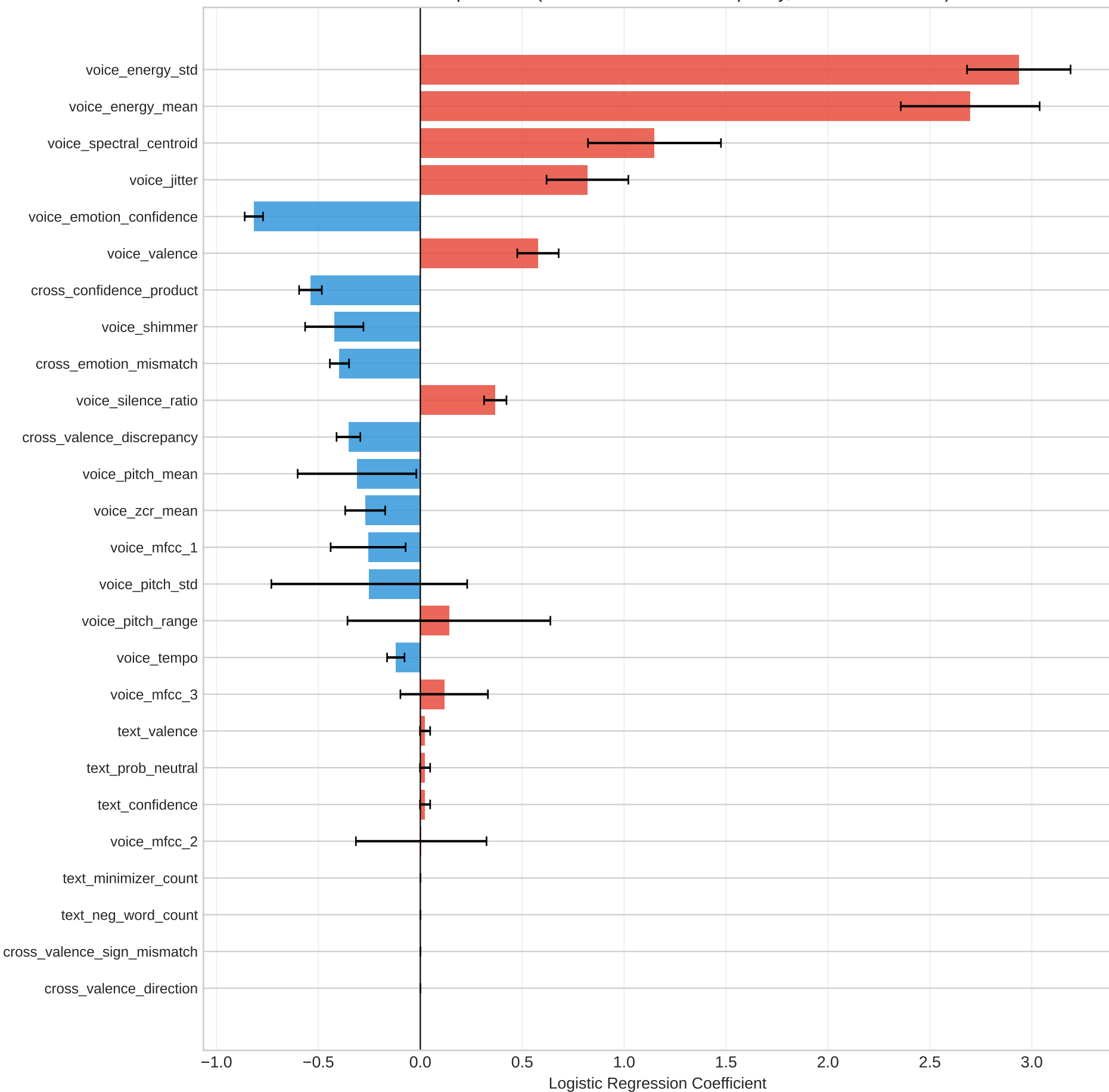
Feature Importance (Red = increases discrepancy, Blue = decreases)
