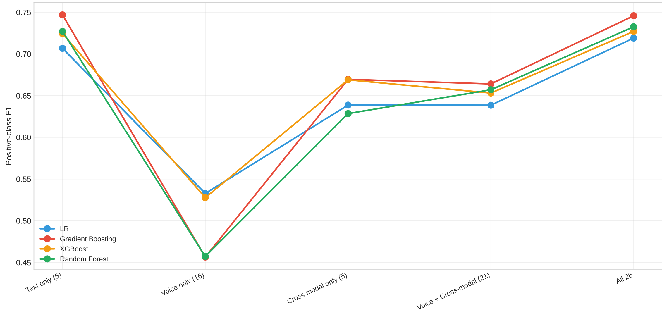
MELD Selection: Feature Subsets
