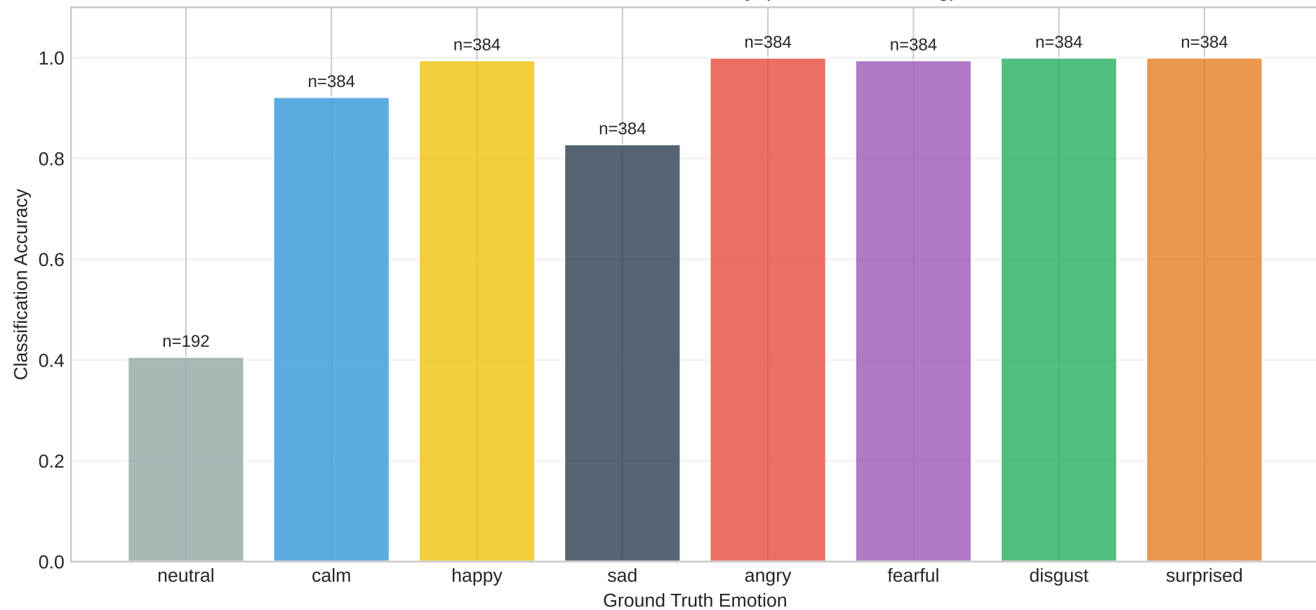
Per-Emotion Detection Accuracy (Gradient Boosting)
