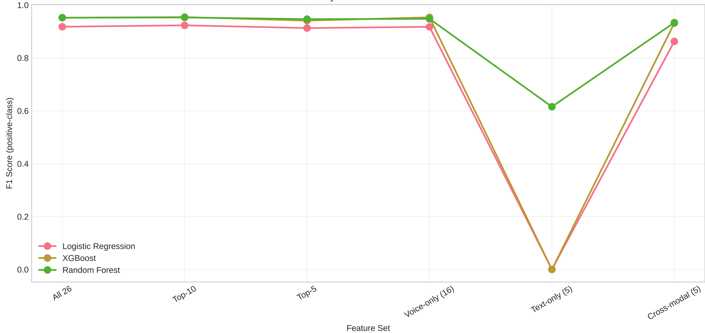
Selection Study: Feature Subsets x Classifiers
