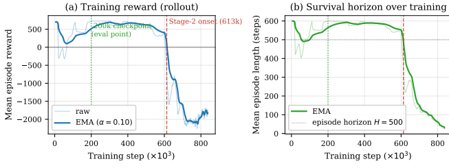
Fig. 4. Training trajectory of the 1.0M-step run. (a) Mean rollout reward per episode (raw + EMA, \alpha=0.10 ). (b) Mean episode length. The green dotted line marks the 200k checkpoint used for Table II; the red dashed line marks the Stage-2 onset at step 613k (rate budget widening from 10^\circ/\text{s} to 15^\circ/\text{s} ).
