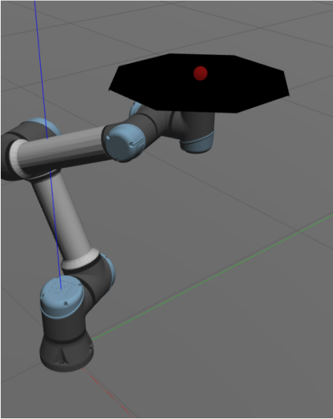
Fig. 2. Experimental setup. A UR5e 6-DOF manipulator carries a 0.70 \times 0.70 m flat plate on its tool flange; a spherical marble of radius 15 mm and mass 50 g rolls on the plate’s top surface. The whole scene is simulated in Gazebo Classic with ODE contact at \mu = 0.6 . The arm tilts the plate via small angular-velocity commands issued through MoveIt 2 Servo to keep the marble centred while the TCP simultaneously traces a 3-D Lissajous disturbance.
