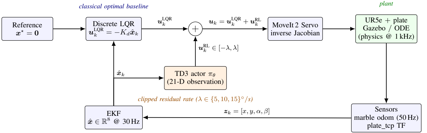
Fig. 1. Hybrid control architecture. The classical baseline (blue) computes u_k^{\text{LQR}} = -K_d \hat{x}_k from the EKF estimate \hat{x}_k \in \mathbb{R}^8 . The learned residual (orange) computes u_k^{\text{RL}} = \pi_\theta(o_k) from a 21-D augmented observation, scaled by the curriculum rate budget \lambda . The two streams sum at the junction and are forwarded to MoveIt 2 Servo at 30 Hz; only the sum reaches the plant. The EKF is the sole bridge between the noisy sensors (marble odometry @ 50 Hz, plate orientation from forward kinematics) and both controllers; numerical differentiation of the TF stream is explicitly avoided in favour of model-based fusion (Sec. III-C).
