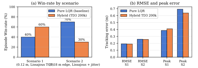
Fig. 2. Head-to-head metrics for Scenarios 1 and 2. Residual TD3 increases nominal-scenario survival rate by 20 percentage points and reduces RMSE by \sim 1\% in both scenarios, but cedes survival authority in the extreme-spawn condition. Numbers reproduced verbatim from Table II.
