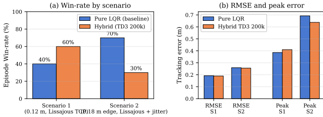
Fig. 3. Head-to-head metrics for Scenarios 1 and 2. Residual TD3 increases nominal-scenario survival rate by 20 percentage points and reduces RMSE by \sim 1\% in both scenarios, but cedes survival authority in the extreme-spawn condition. Numbers reproduced verbatim from Table II.
