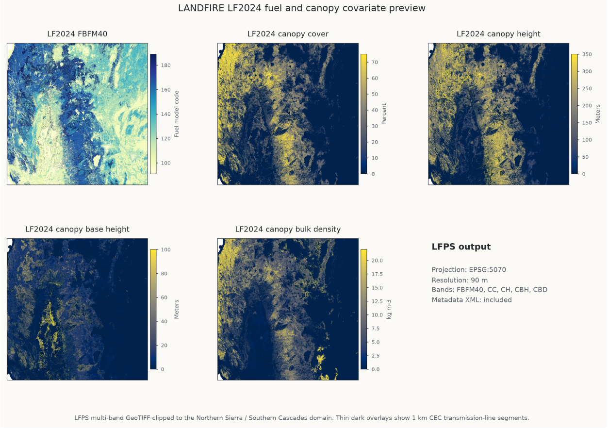
Figure 3: Public environmental covariates used to construct dynamic weather, terrain, and fuel-structure predictors. (c) LANDFIRE LF2024 fuel and canopy covariate preview clipped to the study region.
