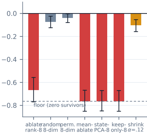
The removal family (naturally-correct rows)
