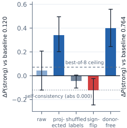
One vector, five fates (failing rows)
