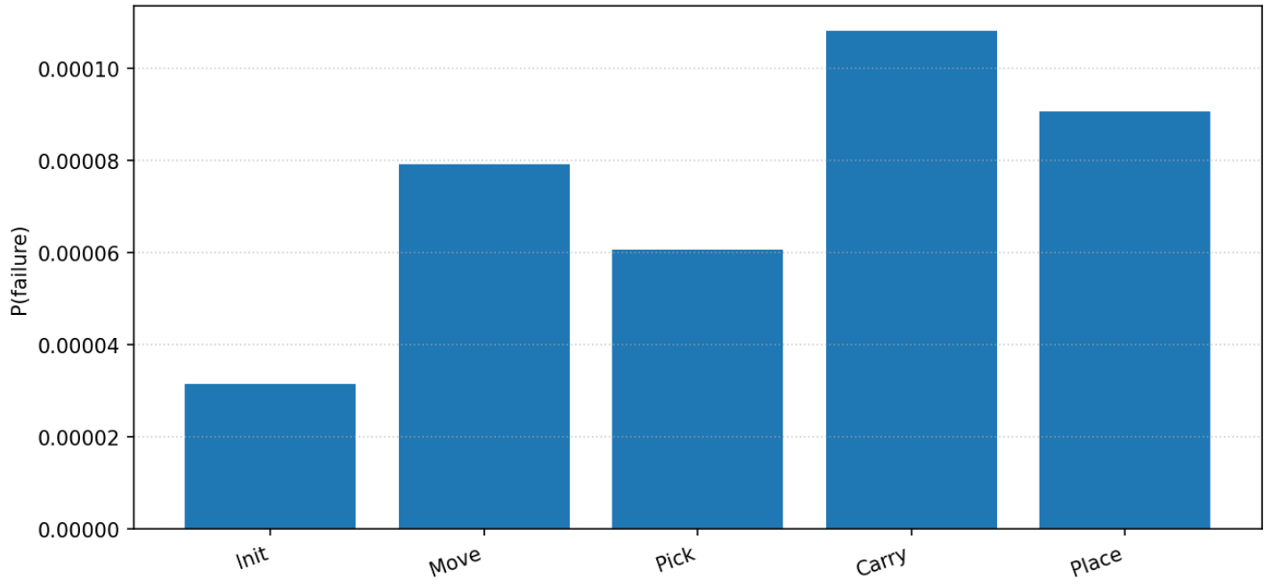
Per-skill failure probability (Absorbing / DTMC)
