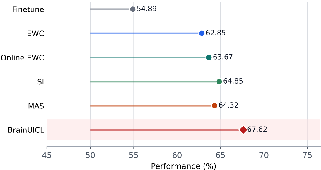
Final Seen New-Subject ACC
