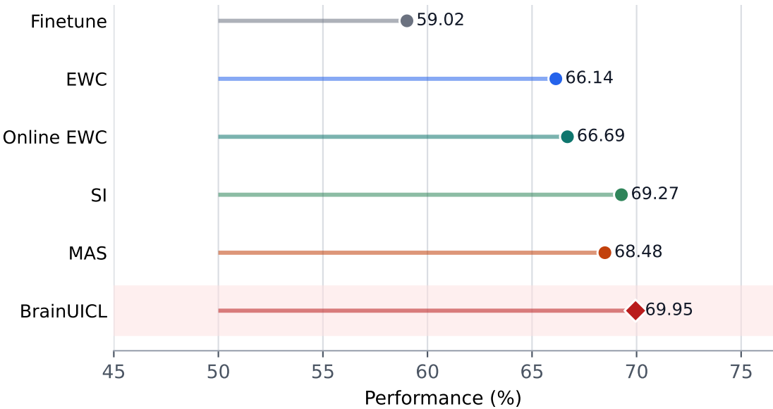
Final Old-Subject Macro-F1
