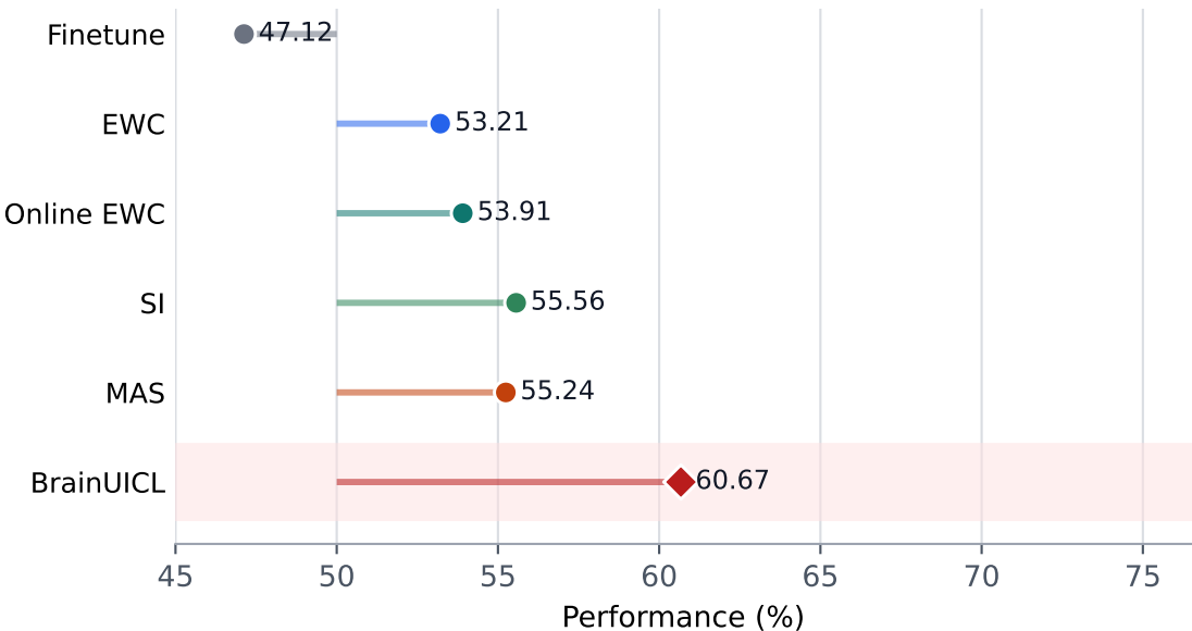
Final Seen New-Subject Macro-F1
