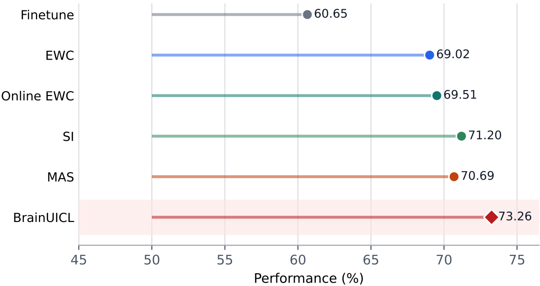
Final Old-Subject ACC
