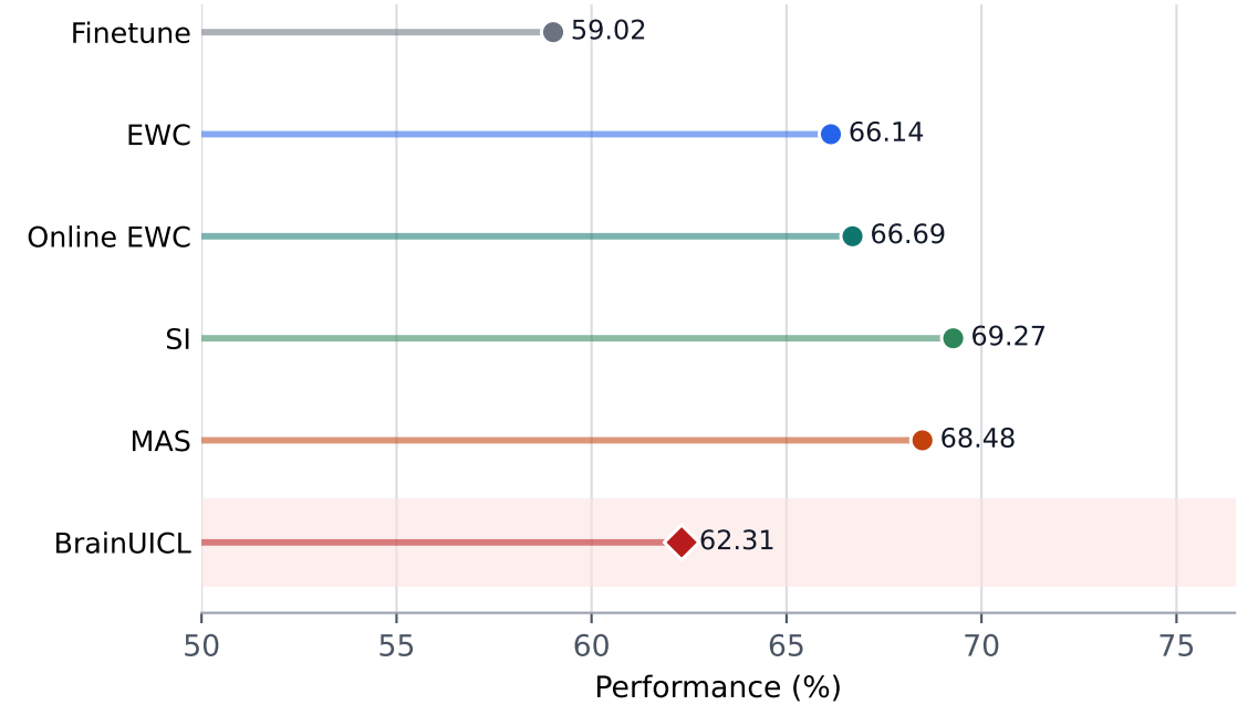
Final Old-Subject Macro-F1
