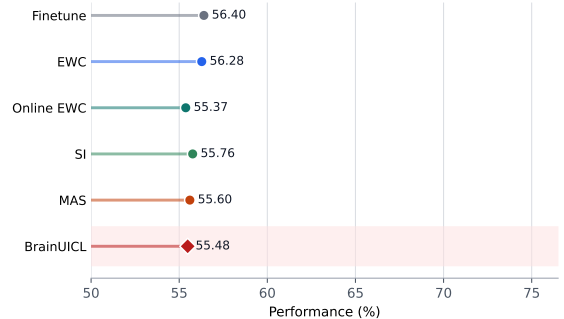
Mean New-Subject Macro-F1 After Adaptation
