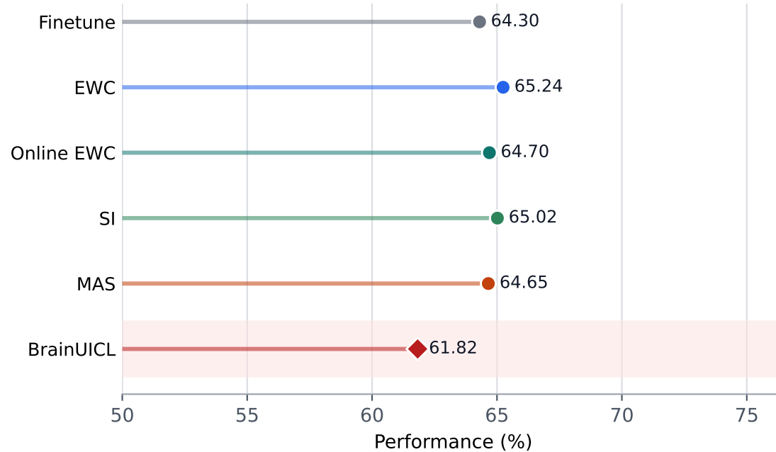
Mean New-Subject ACC After Adaptation
