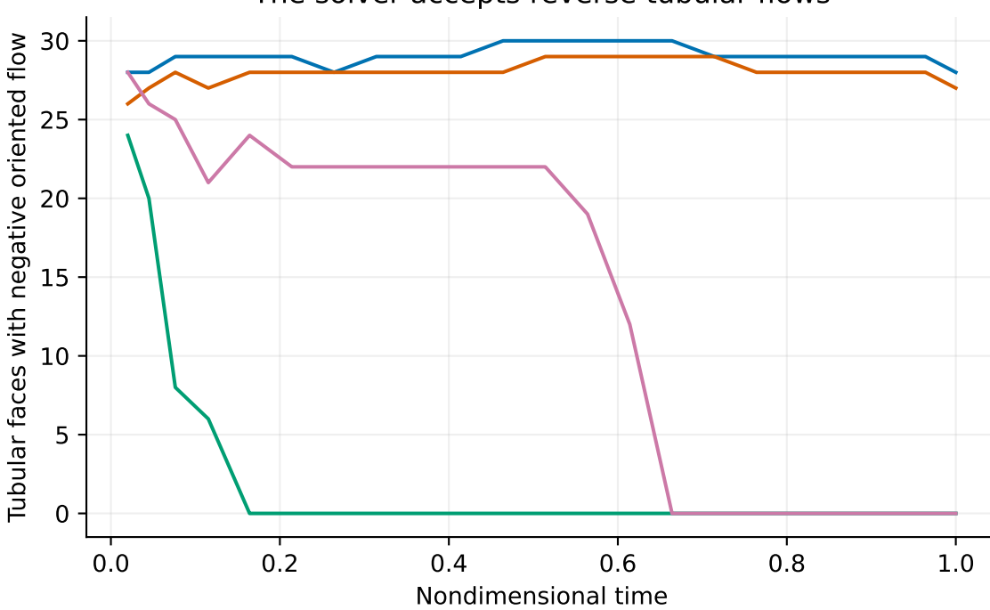
The solver accepts reverse tubular flows
