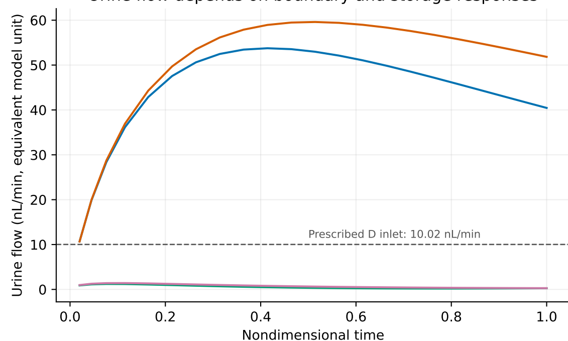
Actual DCT fluxes can violate its transfer rules
