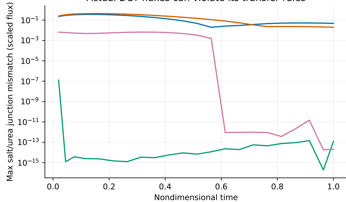
Actual DCT fluxes can violate its transfer rules
