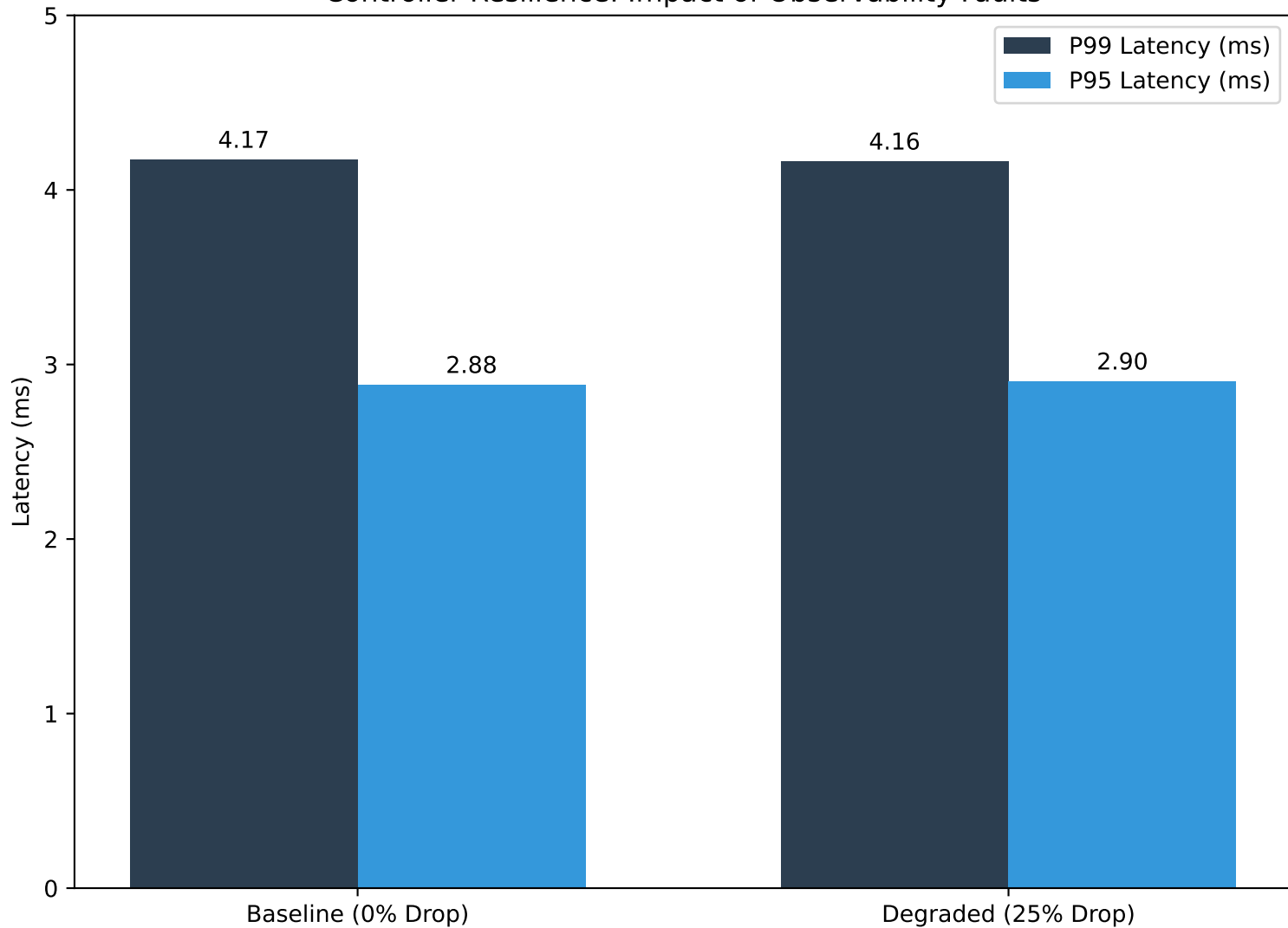
Controller Resilience: Impact of Observability Faults
