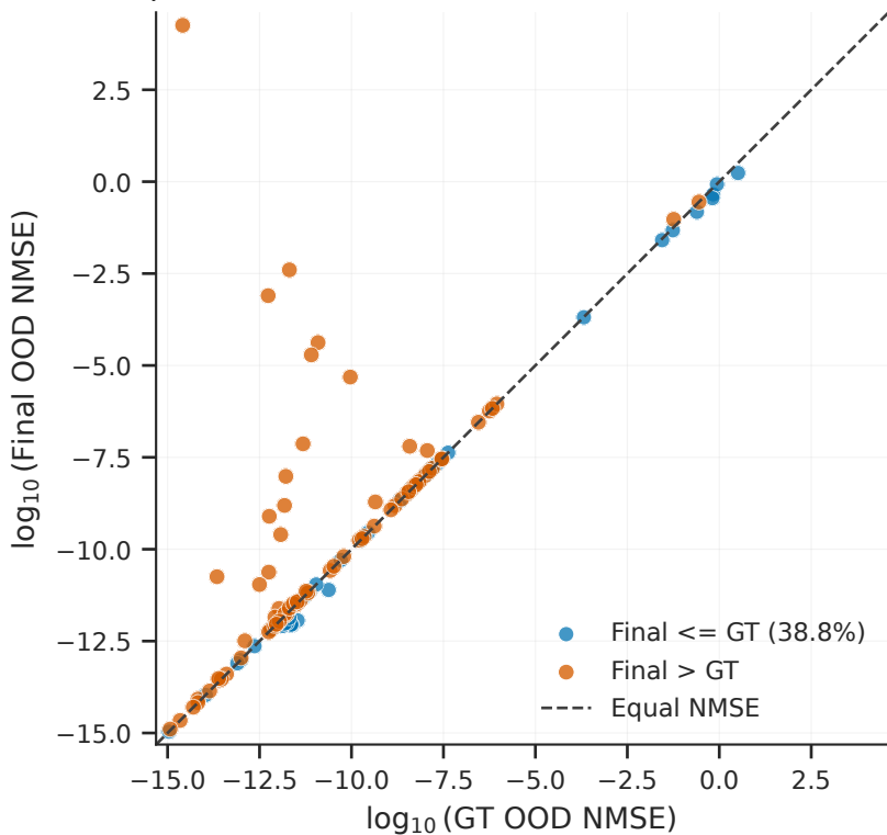
Opus 4.6 Full: Final vs. Ground Truth (OOD NMSE)
