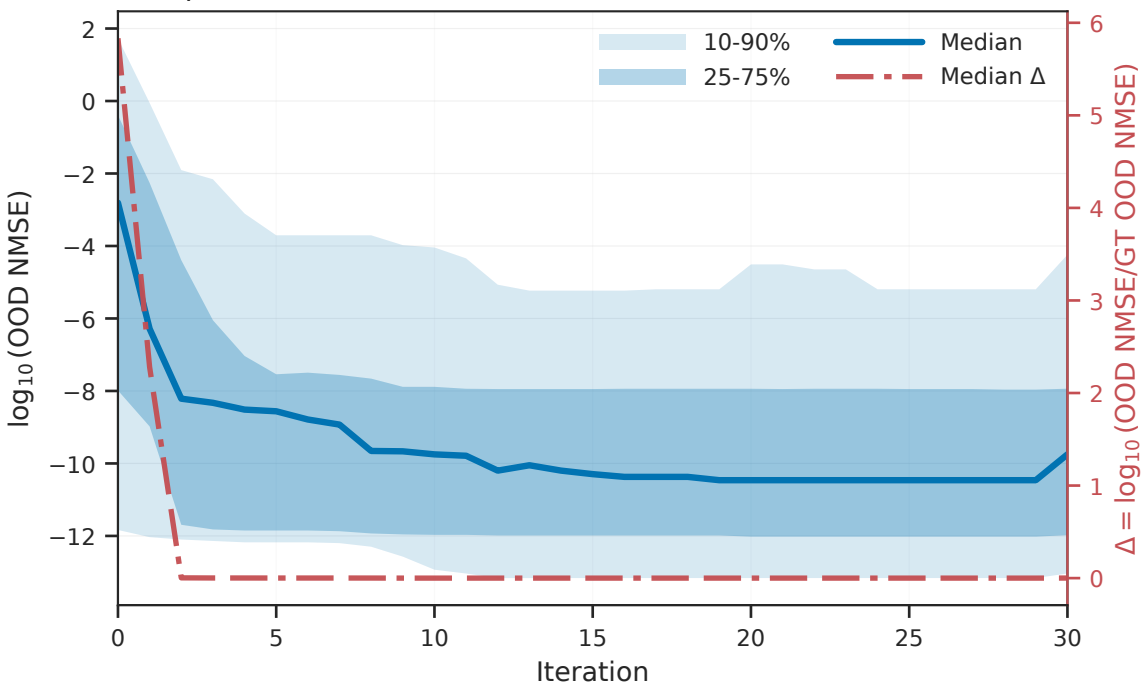
Opus 4.6 Full: Global-Best OOD NMSE Distribution (n=129)
