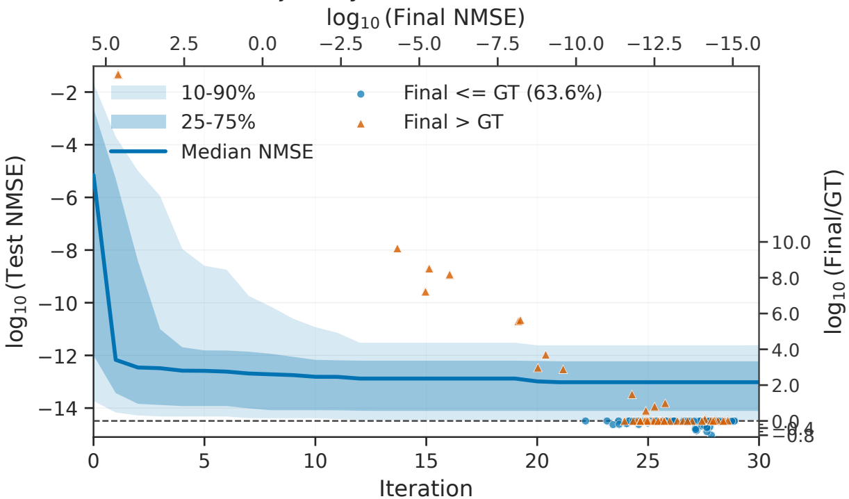
Test NMSE trajectory with final relative-error scatter
