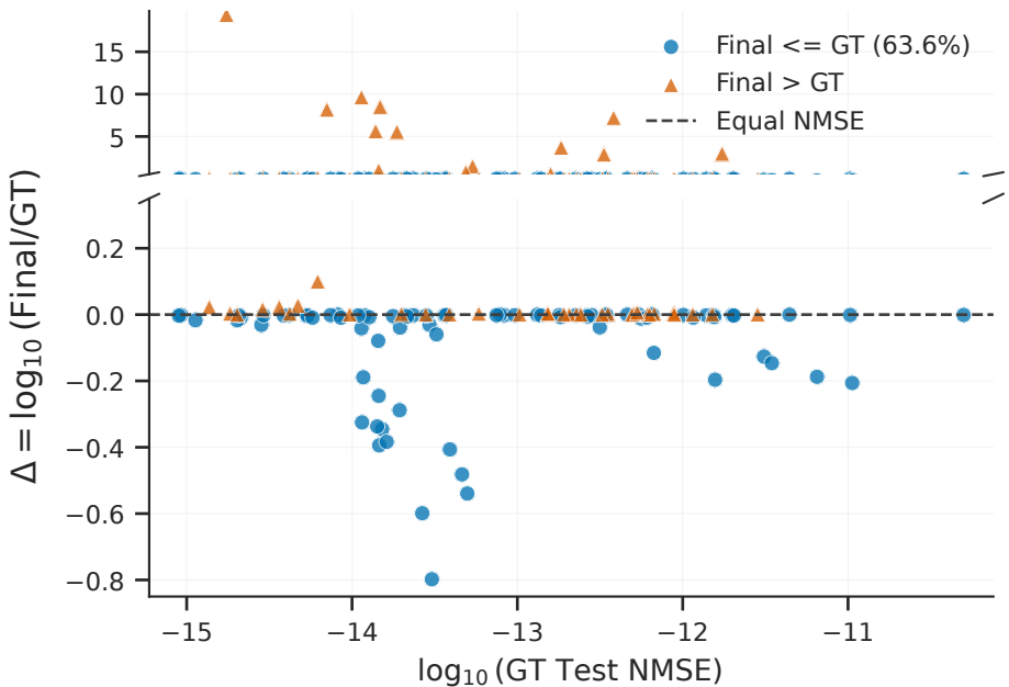
Opus 4.6 Full: Relative Test NMSE
