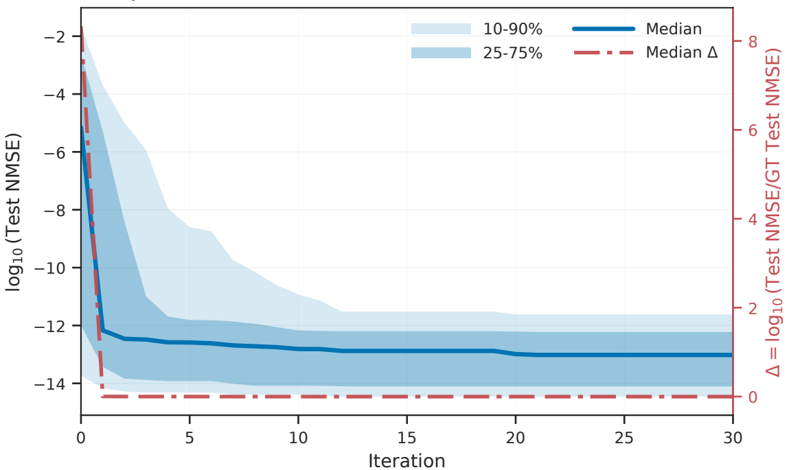
Opus 4.6 Full: Global-Best Test NMSE Distribution (n=129)
