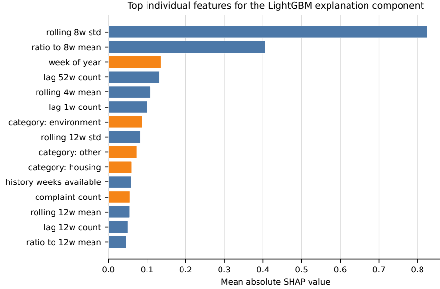
Fig. 4 Top 15 individual features by mean absolute SHAP value for the tuned LightGBM explanation component. Blue bars are historical temporal features; orange bars are other feature groups.
