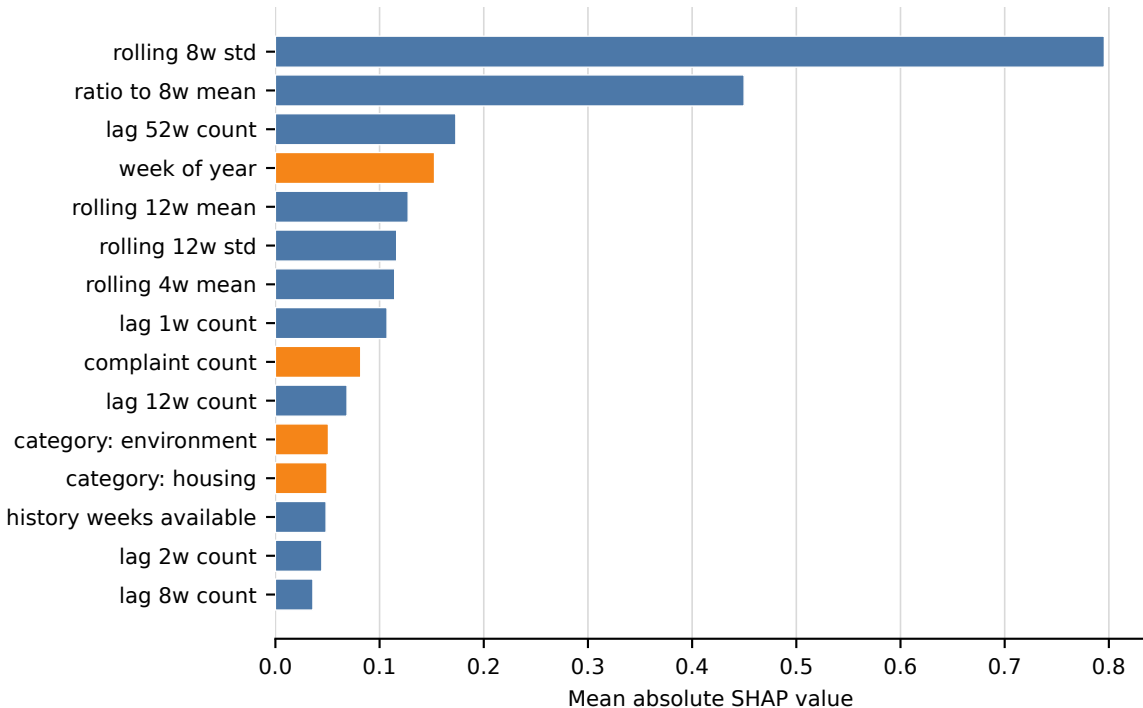
Top individual features for the LightGBM explanation component
