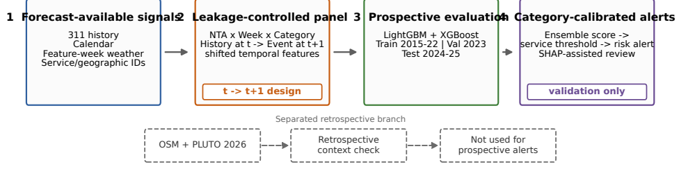
Fig. 1 Overview of the revised early-warning framework. The prospective alerting path uses only predictors available by the end of feature week t , while the target represents abnormal reported demand at t + 1 . Models are evaluated chronologically, and category thresholds are selected on validation. Contemporary OSM and PLUTO snapshots are assessed separately as retrospective context and are not used to produce prospective alerts.
