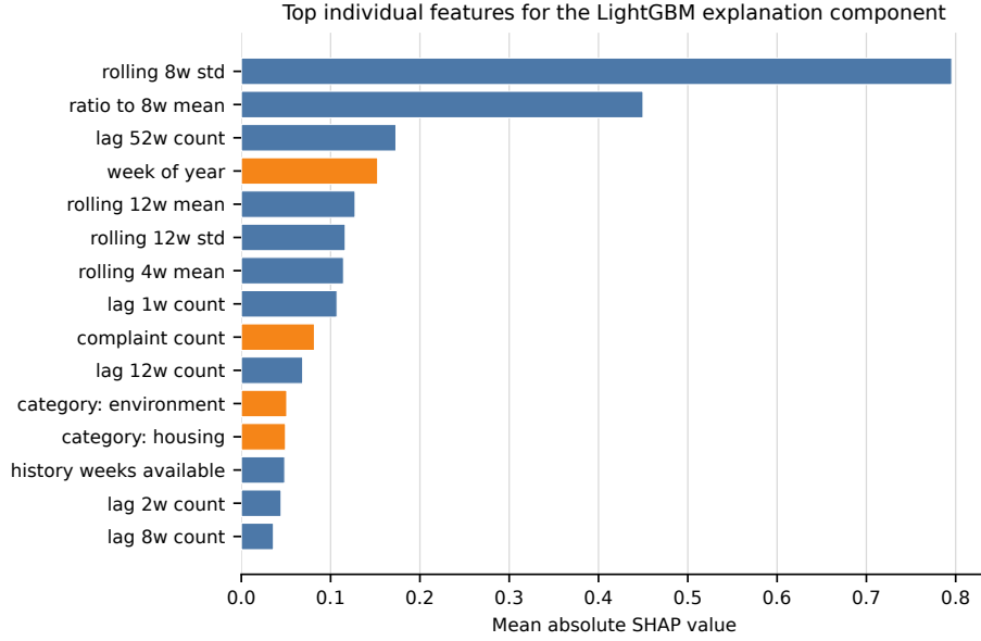
Fig. 4 Top individual SHAP features for the prospective LightGBM explanation component. Blue bars are historical temporal features; orange bars are other feature groups.
