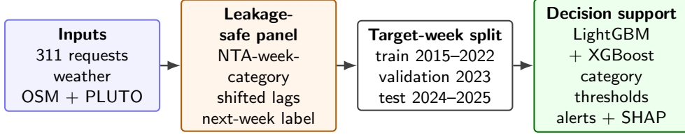
Fig. 1 End-to-end leakage-safe workflow. Feature week t predicts target week t + 1 ; chronological periods are split by target week before fitting; thresholds are selected only on validation; and SHAP reports normalized summed mean absolute contribution patterns for reported demand rather than causal effects.
