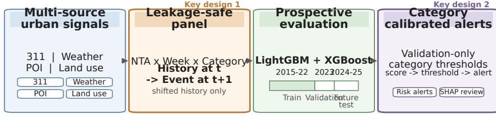
Fig. 1 Overview of the proposed early-warning framework. Multi-source urban signals are organized into a leakage-safe NTA-week-category panel, where information available at week t predicts abnormal reported demand at t+1 . Models are evaluated prospectively, and validation-only category thresholds convert ensemble scores into service-specific alerts. SHAP supports post-hoc analyst review.
