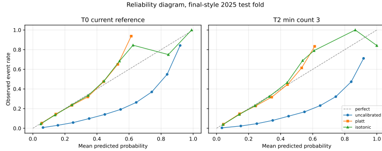
Fig. 1 Reliability diagram for the final-style calibrated LightGBM candidate. Calibration is fit on validation year 2024 and evaluated unchanged on held-out year 2025.
