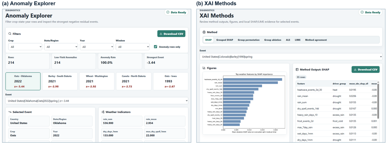
Fig. 9. Web prototype views. The anomaly explorer filters crop-state-year rows and highlights the strongest low-yield residual events, while the XAI view exposes feature- and driver-group evidence for selected cases.
