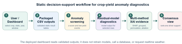
Fig. 8. Decision-support prototype architecture. The dashboard consumes static validated outputs and exposes anomaly screening, residual-model diagnostics, multi-method XAI evidence, and consensus summaries without retraining or real-time weather queries.
