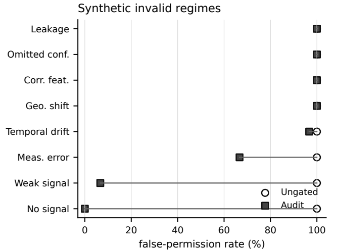
Fig. 3. Synthetic calibration of ungated explanation permission versus the observable A+B+E audit rule across structurally invalid regimes. GT labels are used only for evaluation, not as inputs to the audit decision.
