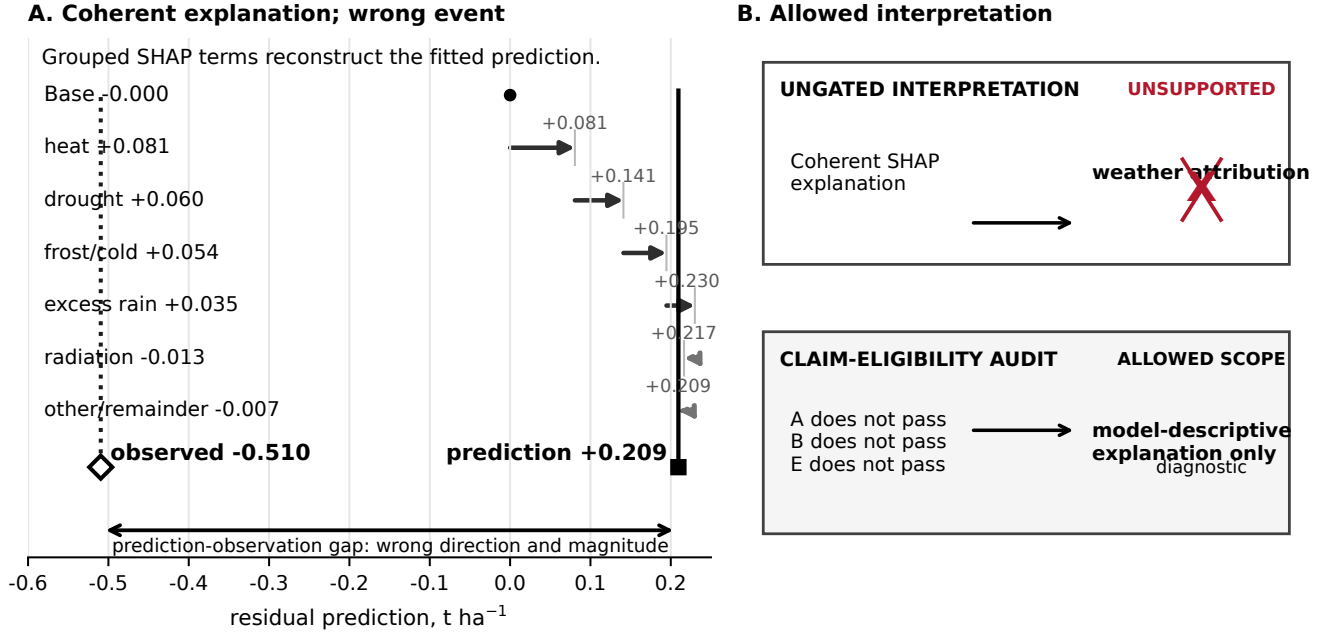
Fig. 2. A coherent explanation of an ineligible prediction. (A) For the locked Weather-only Barley–Colorado 2016 row, the unrounded grouped SHAP terms reconstruct the fitted prediction of +0.209 , while the observed residual is -0.510 \text{ t ha}^{-1} . Displayed values are rounded, and unrounded terms reconstruct the fitted prediction. The explanation therefore describes how the model reached its prediction, not the observed event. (B) Ungated interpretation would promote the explanation to a weather-attribution claim; the claim-eligibility audit retains it only as a model-descriptive diagnostic because Modules A, B, and E do not pass.
