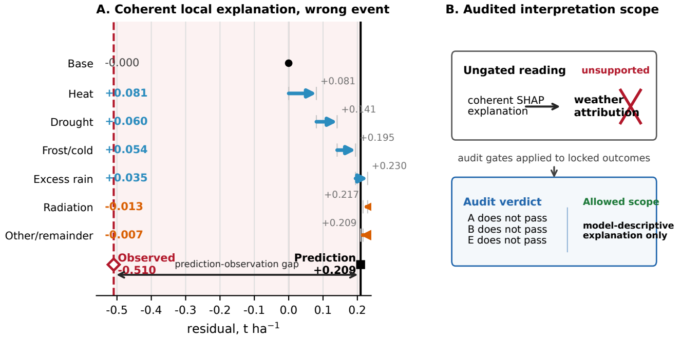
Fig. 2. A coherent explanation of an ineligible prediction. (A) For the locked Weather-only Barley–Colorado 2016 row, the unrounded grouped SHAP terms reconstruct the fitted prediction of +0.209, while the observed residual is -0.510\ t\ ha^{-1} . Displayed values are rounded, and unrounded terms reconstruct the fitted prediction. The explanation therefore describes how the model reached its prediction, not the observed event. (B) Ungated interpretation would promote the explanation to a weather-attribution claim; the claim-eligibility audit retains it only as a model-descriptive diagnostic because Modules A, B, and E do not pass.
