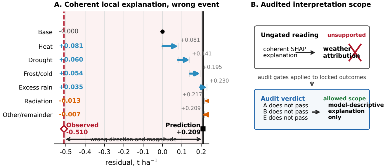
Fig. 2. A coherent explanation of an ineligible prediction. (A) For the locked Weather-only Barley–Colorado 2016 row, the unrounded grouped SHAP terms reconstruct the fitted prediction of +0.209 , while the observed residual is -0.510\ t\ ha^{-1} . Displayed values are rounded, and unrounded terms reconstruct the fitted prediction. The explanation therefore describes how the model reached its prediction, not the observed event. (B) Ungated interpretation would promote the explanation to a weather-attribution claim; the claim-eligibility audit retains it only as a model-descriptive diagnostic because Modules A, B, and E do not pass.
