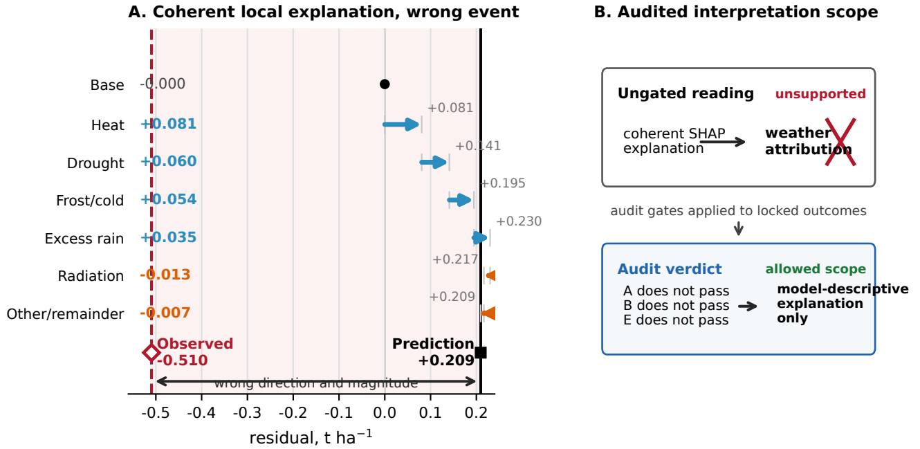
Fig. 2. A coherent explanation of an ineligible prediction. (A) For the locked Weather-only Barley–Colorado 2016 row, the unrounded grouped SHAP terms reconstruct the fitted prediction of +0.209 , while the observed residual is -0.510\ t\ ha^{-1} . Displayed values are rounded, and unrounded terms reconstruct the fitted prediction. The explanation therefore describes how the model reached its prediction, not the observed event. (B) Ungated interpretation would promote the explanation to a weather-attribution claim; the claim-eligibility audit retains it only as a model-descriptive diagnostic because Modules A, B, and E do not pass.
