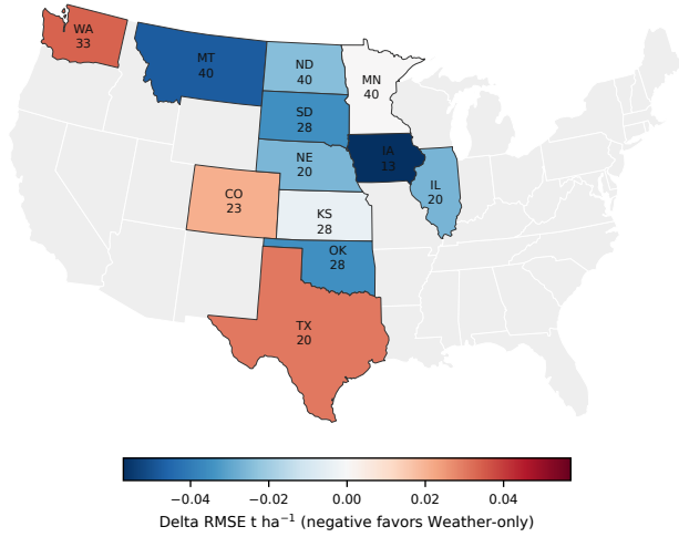
Fig. 4. State-level heterogeneity on the locked 2016–2025 crop panel. Colors show Weather-only minus zero-residual \Delta\text{RMSE} ; negative values favor Weather-only. Labels report state abbreviation and locked-row count. Gray states are outside the study panel. Subgroup estimates are descriptive and not separate module decisions.
