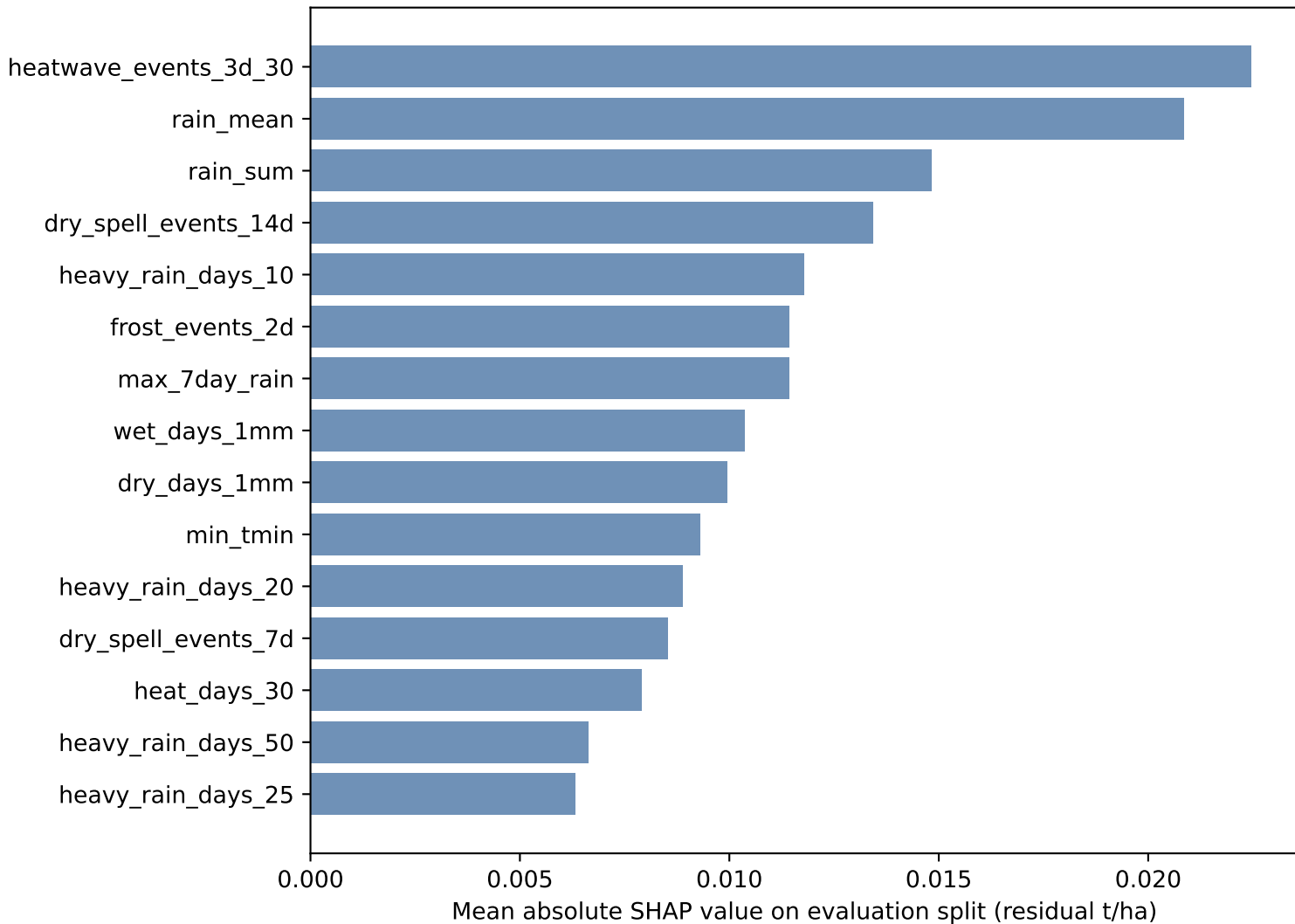
Top weather features by SHAP importance
