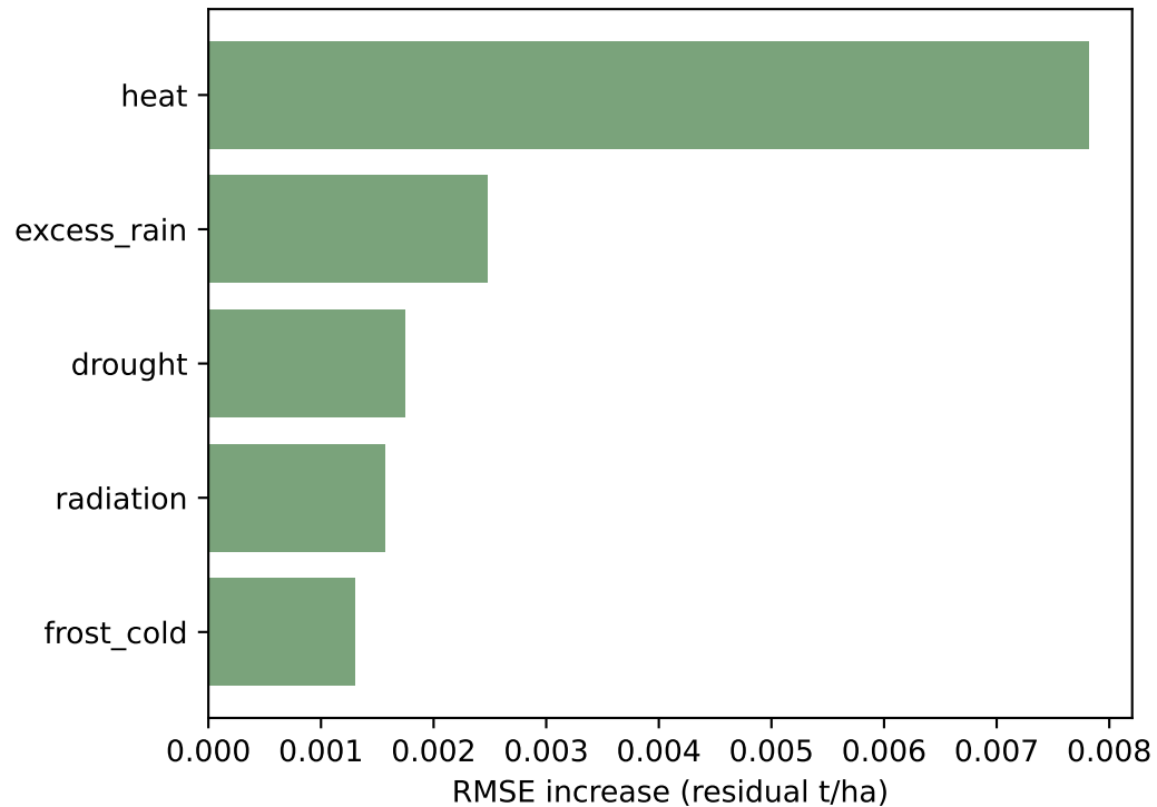
Group ablation
