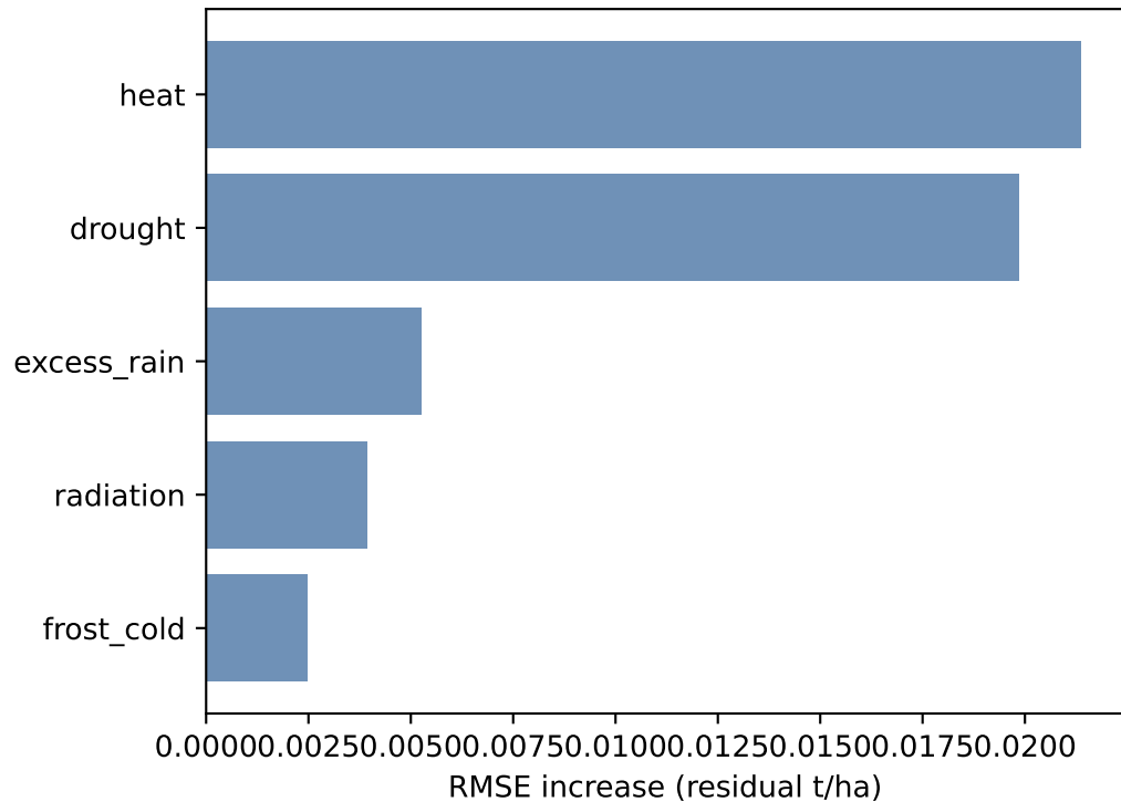
Group permutation
