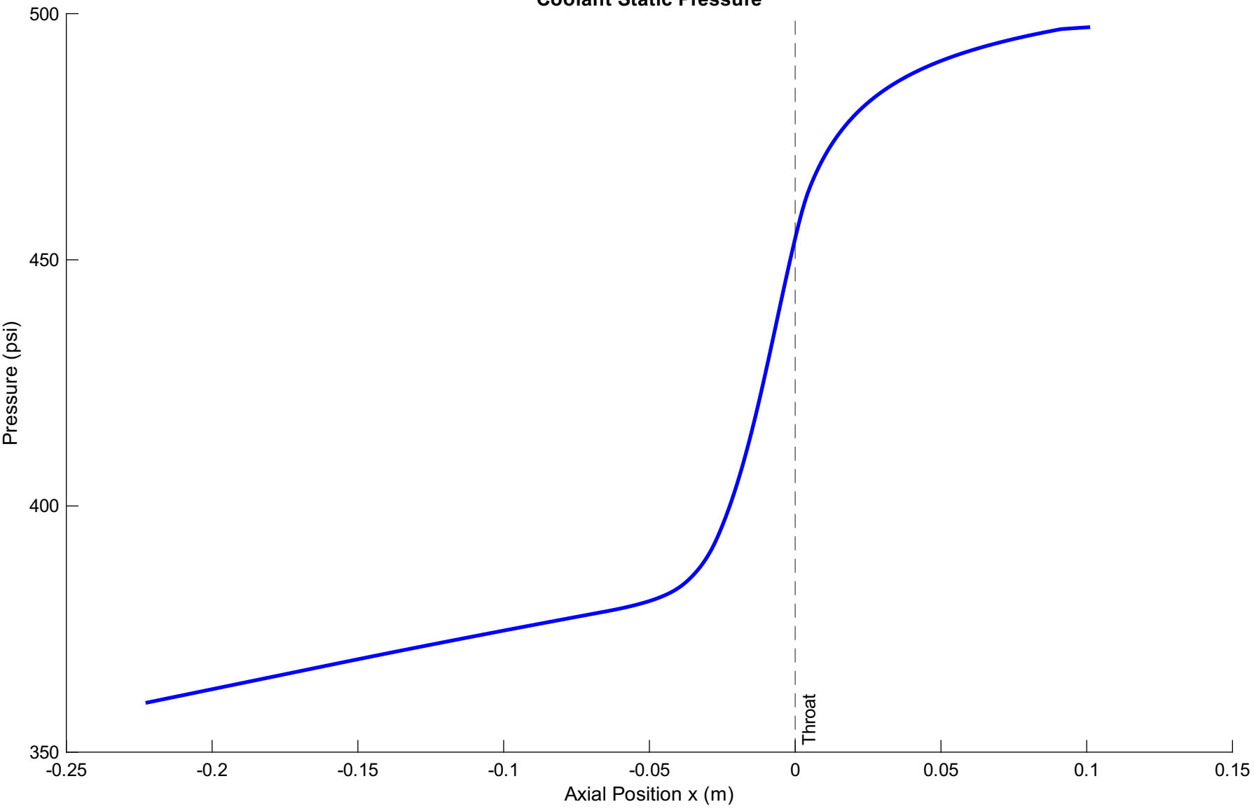
Coolant Static Pressure
