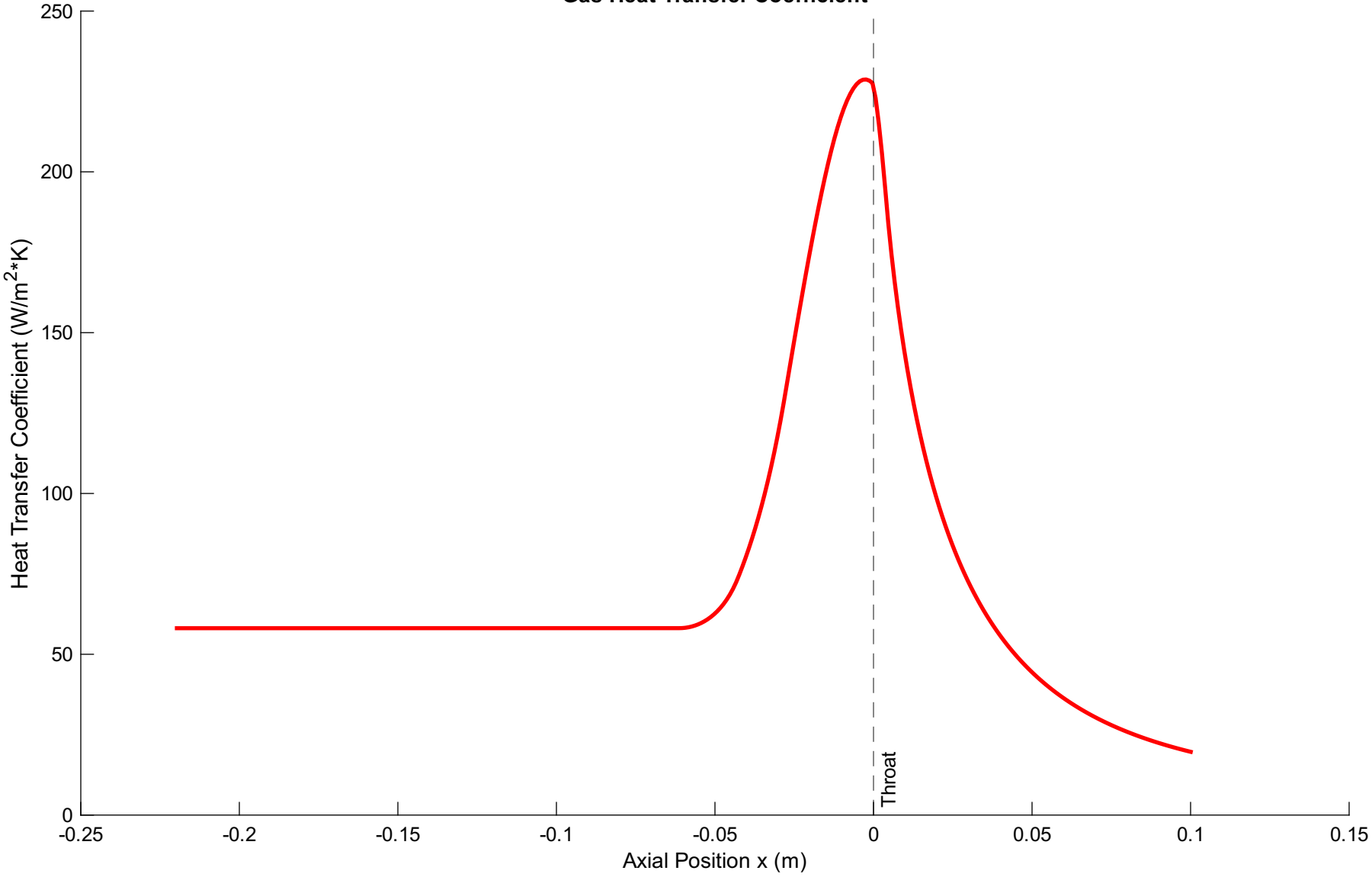
Gas Heat Transfer Coefficient
