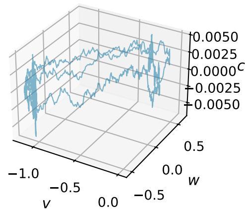
(c) 3D trajectory ( v, w, c )
