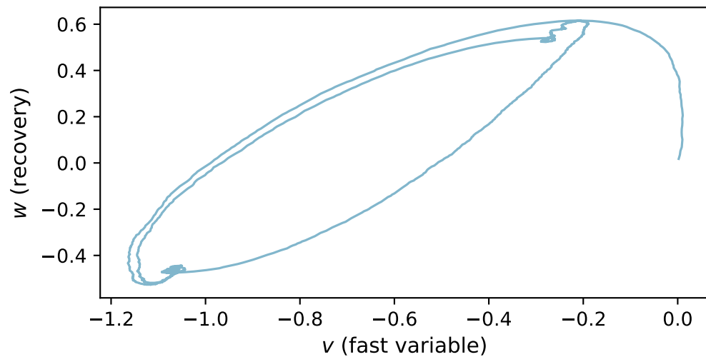
(b) Phase portrait ( v, w )
