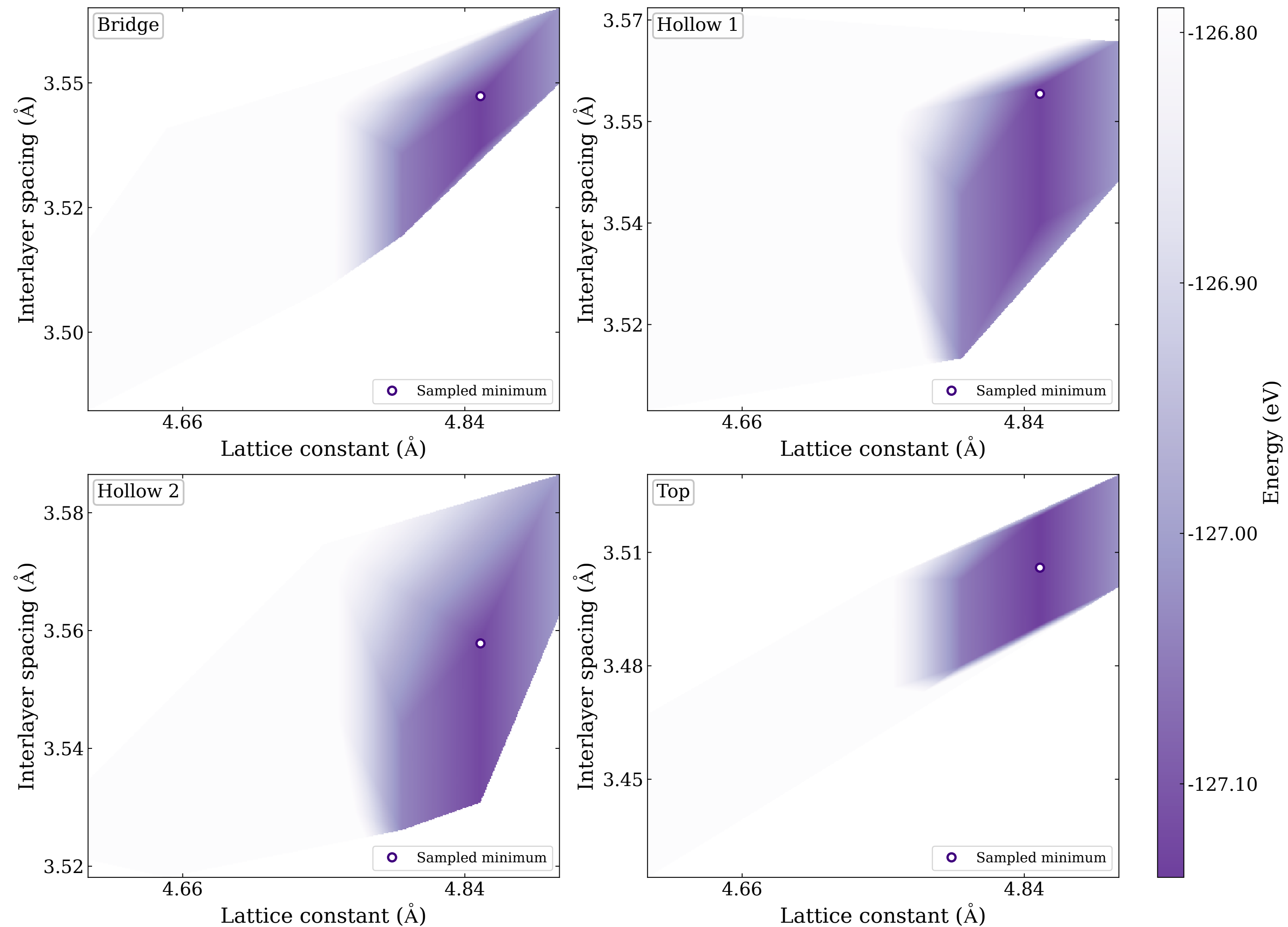
Total energy versus lattice and interlayer spacing for Graphene-B 4 C 3
