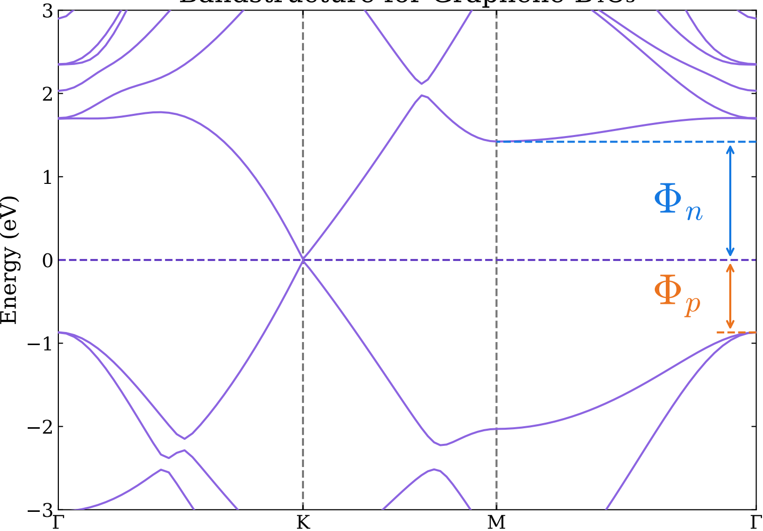
Bandstructure for Graphene-B 4 C 3
