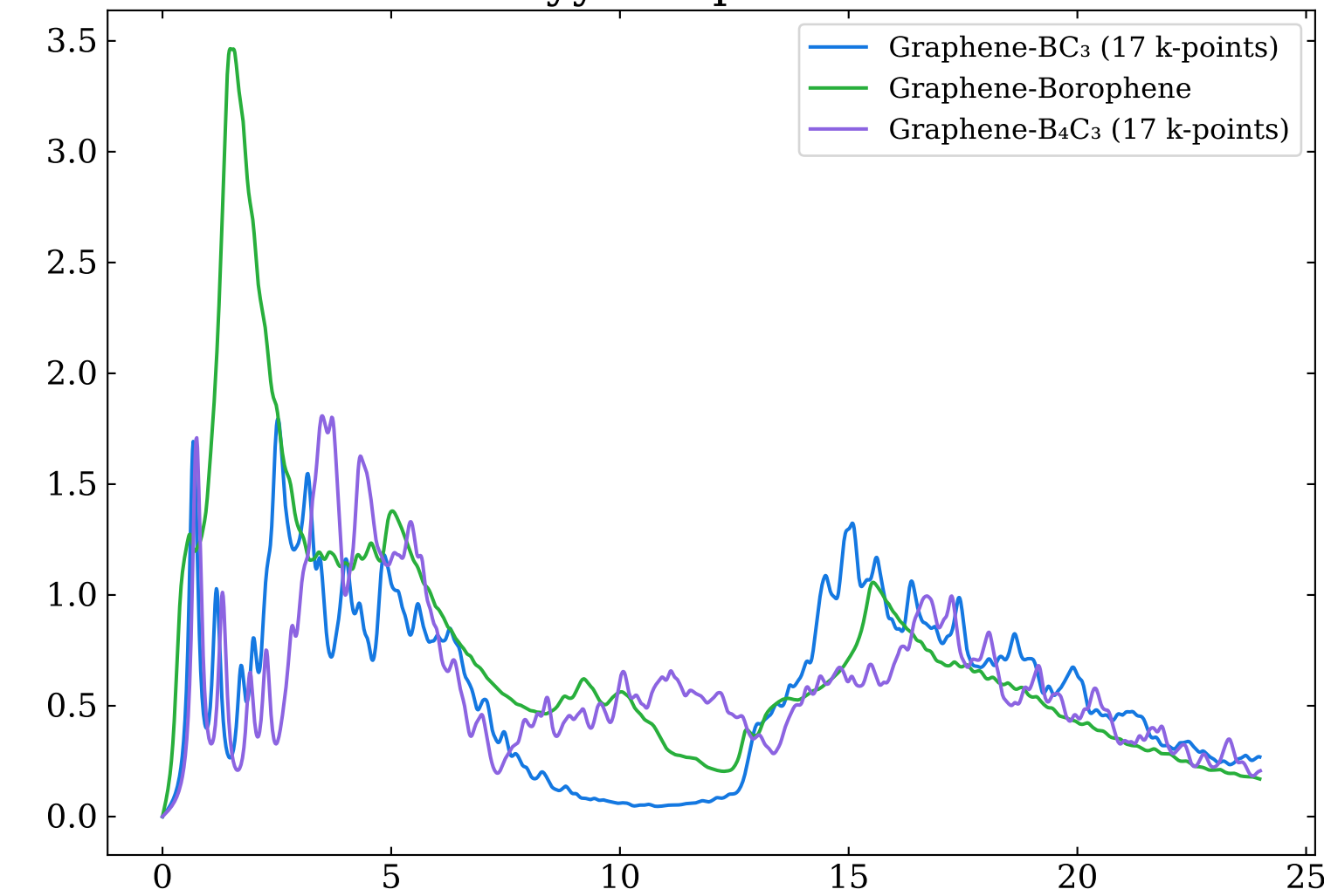
Extinction coefficient for bilayers by HSE06
