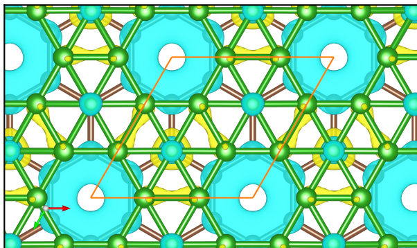
(b) Graphene-Borophene
