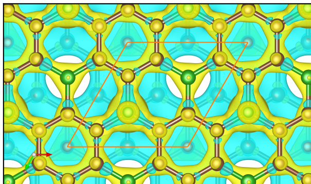
(a) Graphene-BC 3
