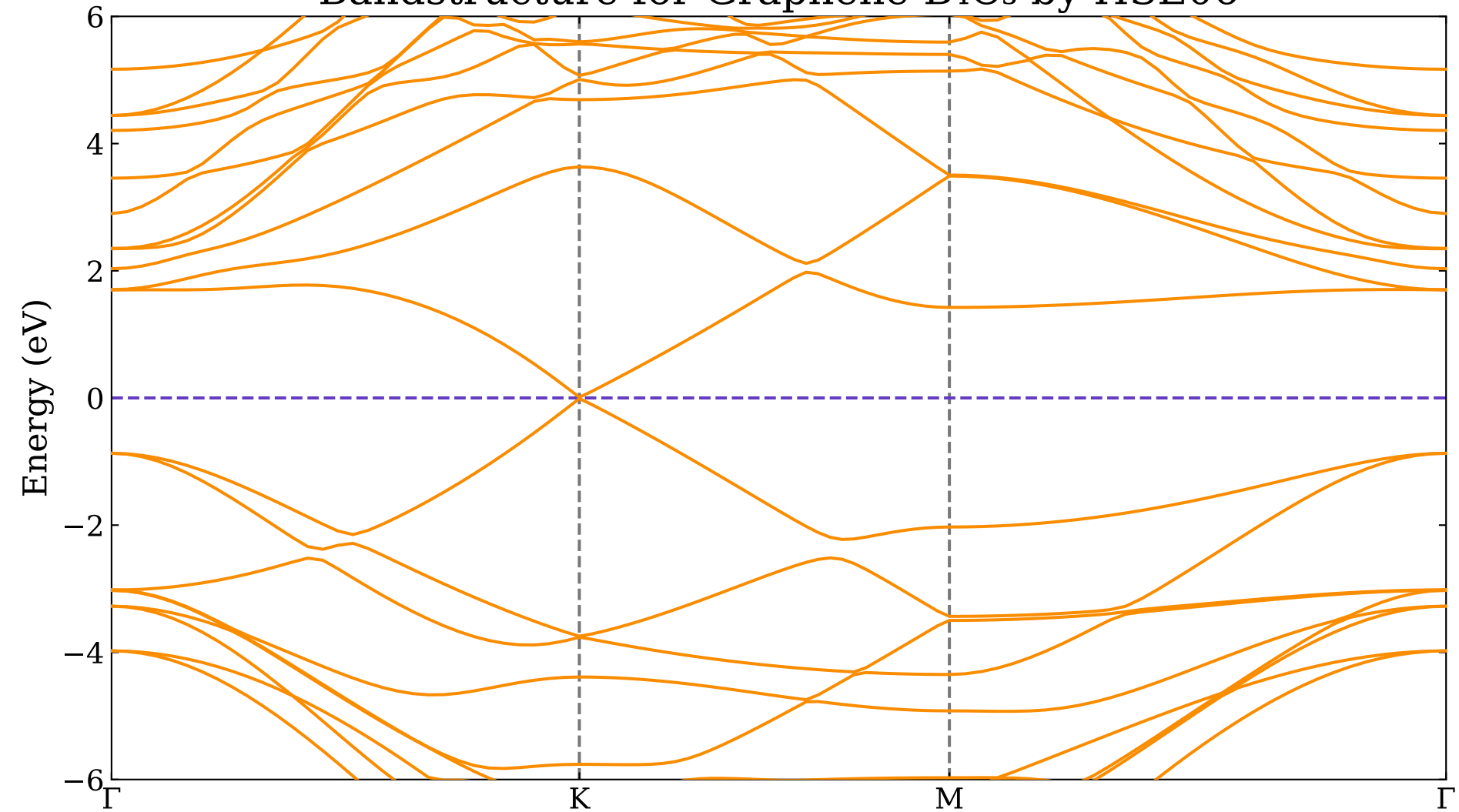
Bandstructure for Graphene-B 4 C 3 by HSE06
