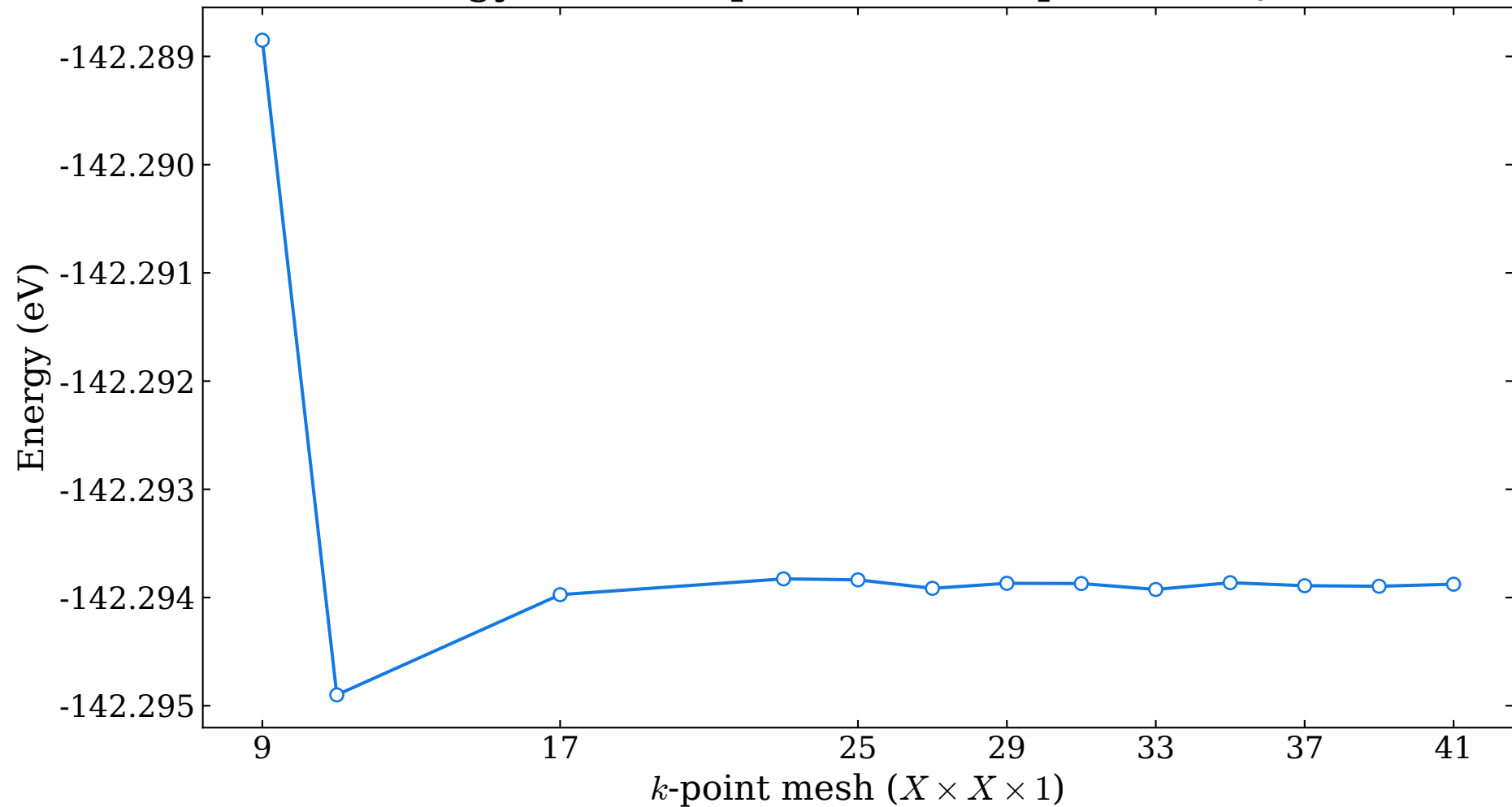
Total energy versus k-points for Graphene-BC 3 (Hollow)
