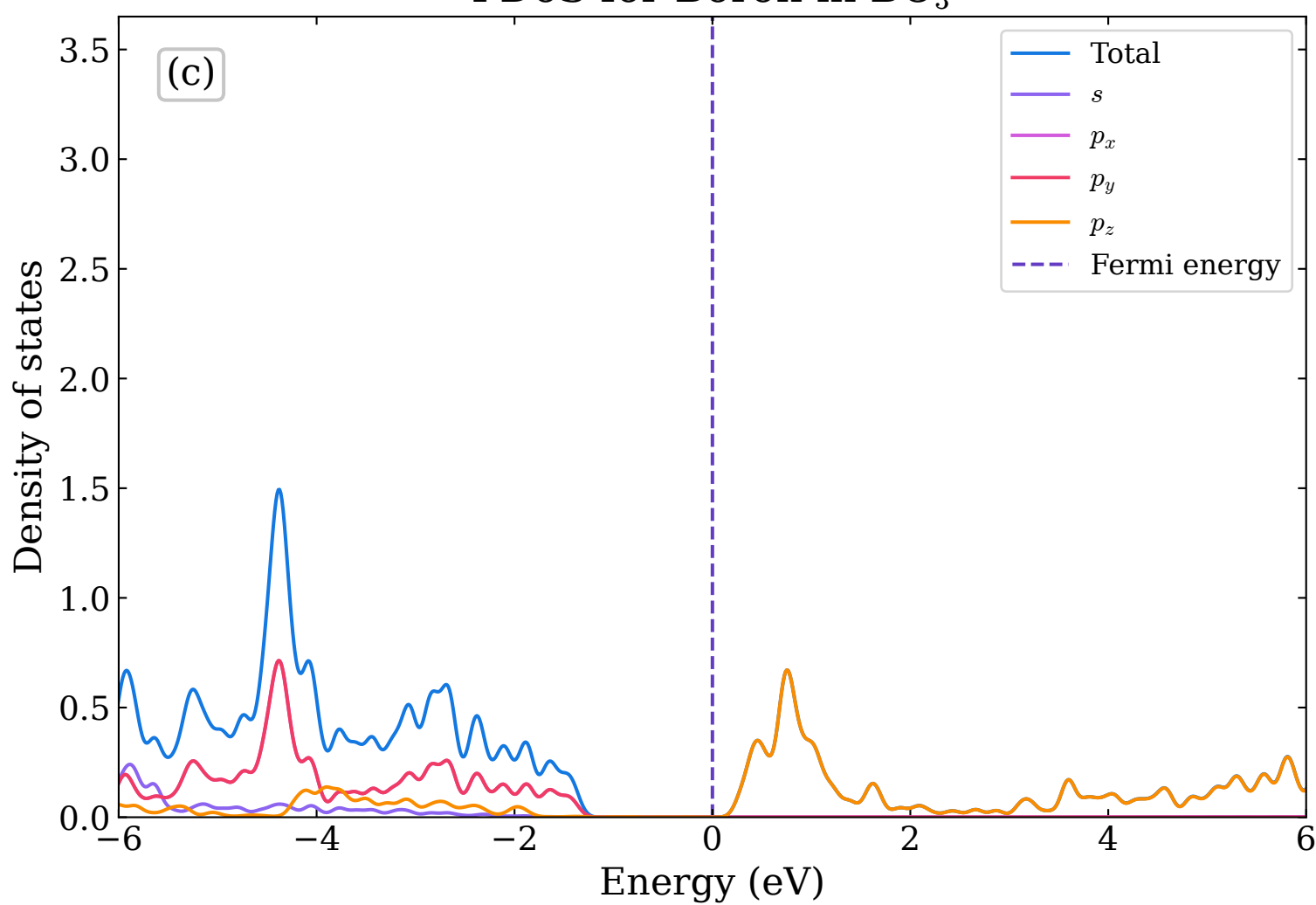
PDoS for Boron in BC 3
