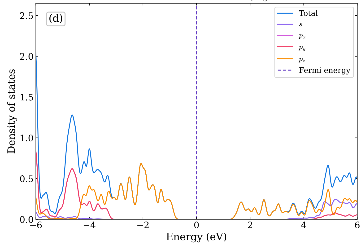
PDoS for Carbon in B 4 C 3
