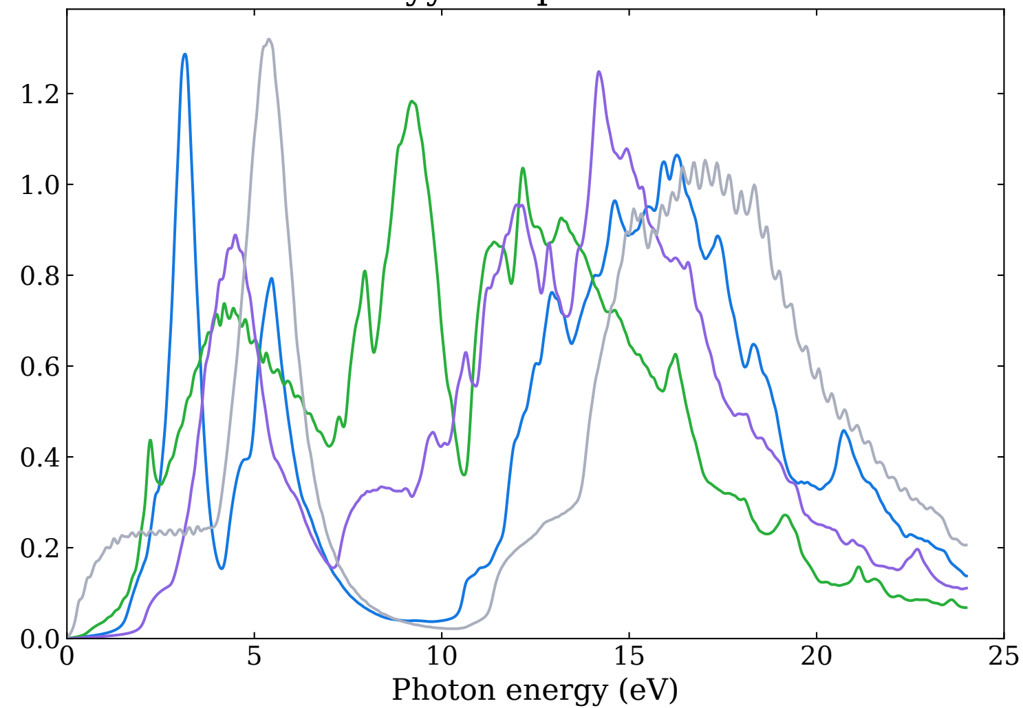
Energy-loss spectrum for monolayers by PBE in-plane yy-component
