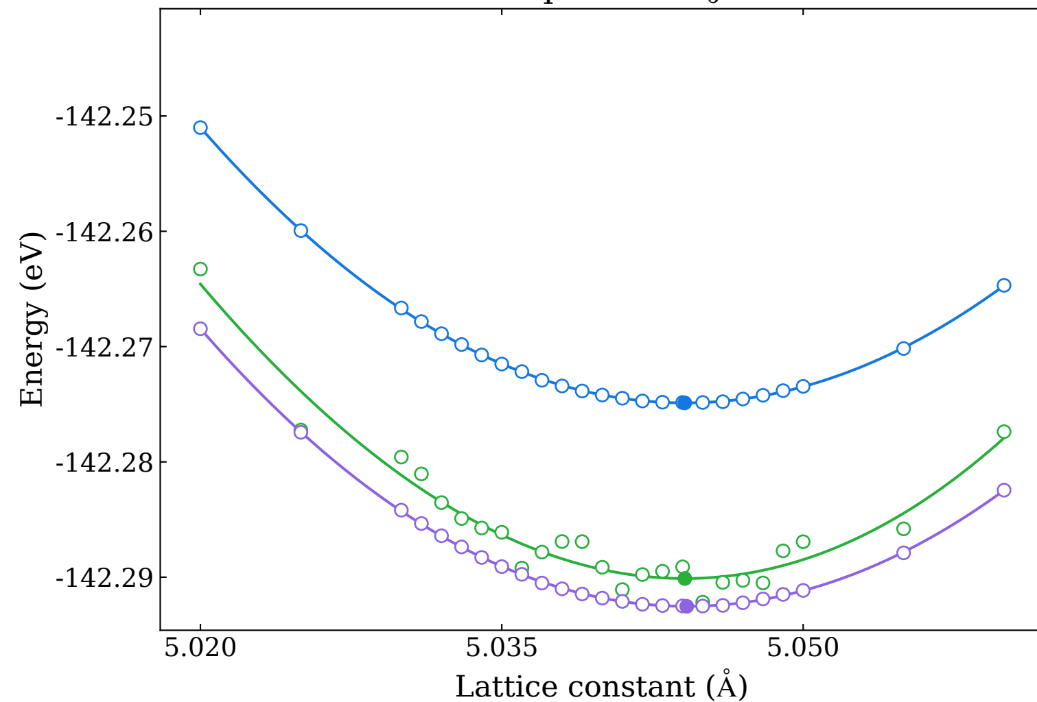
Graphene-B 4 C 3
