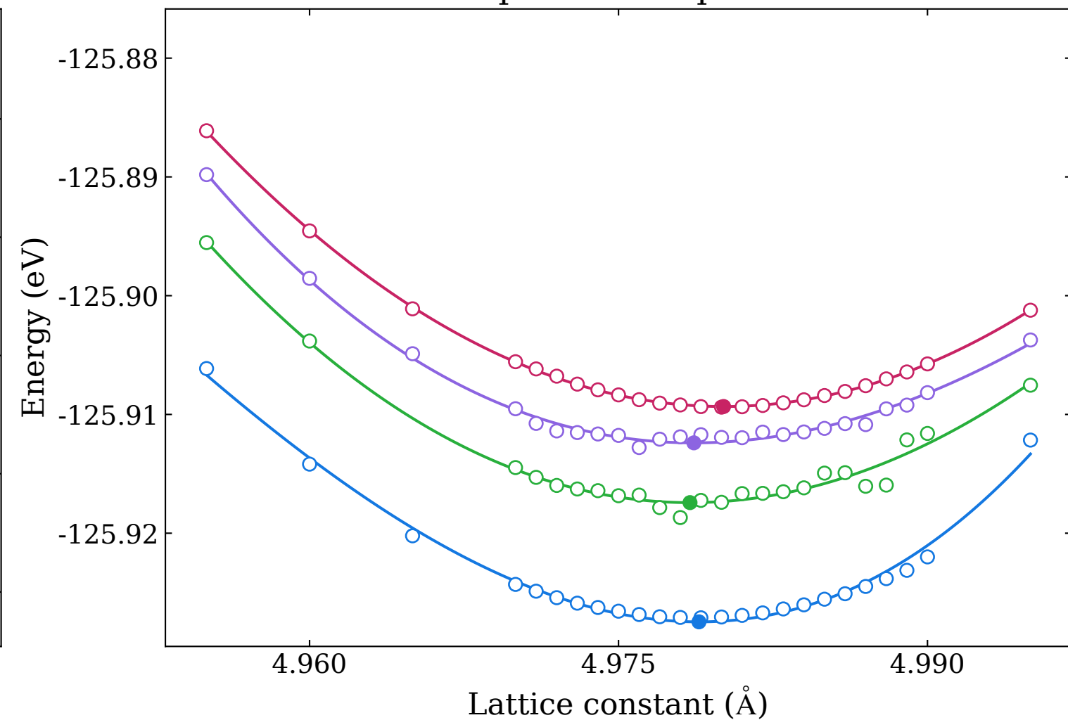
Graphene-Borophene
