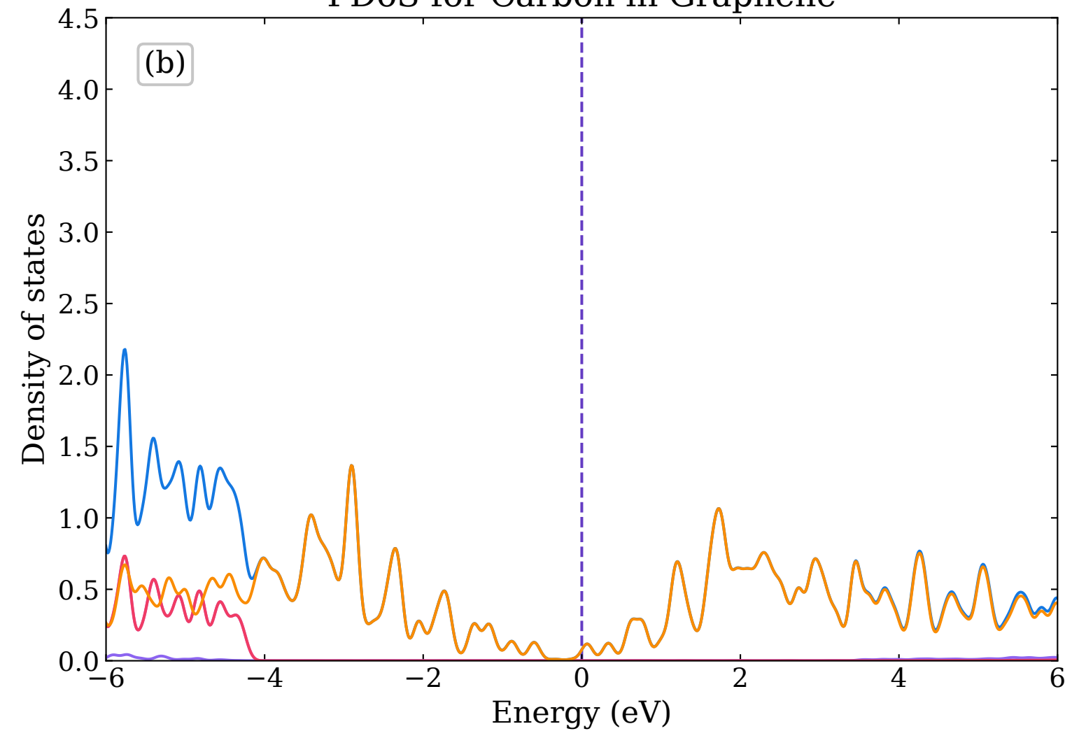
PDoS for Carbon in Graphene
