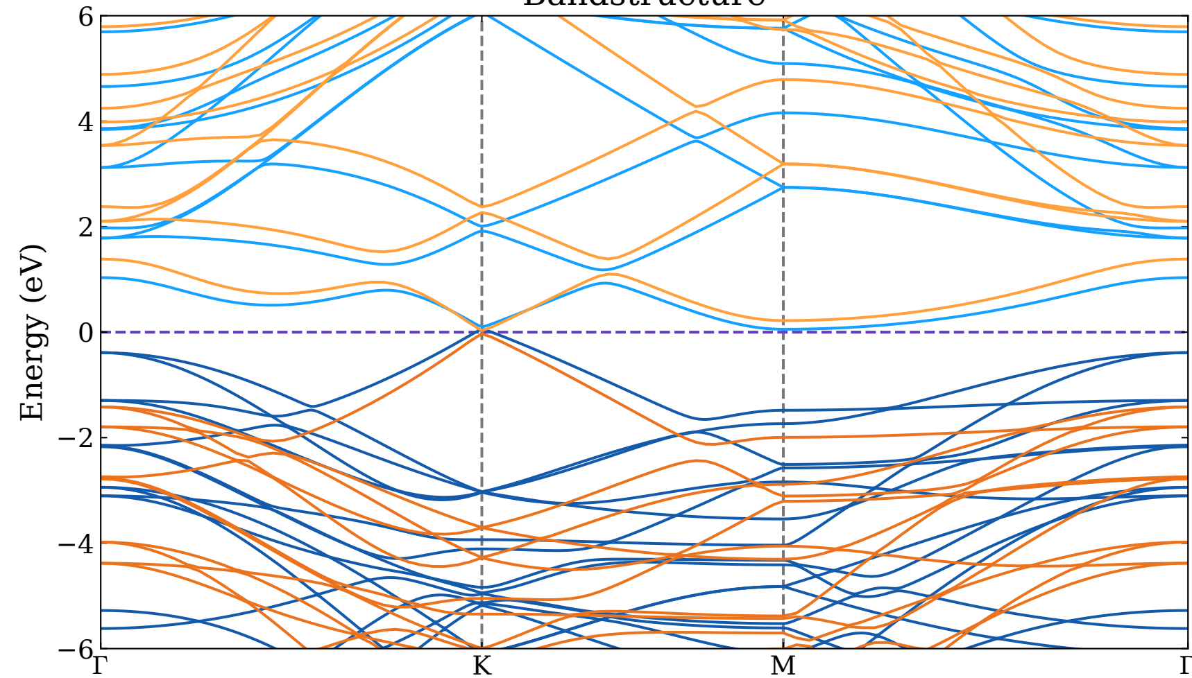
Bandstructure
