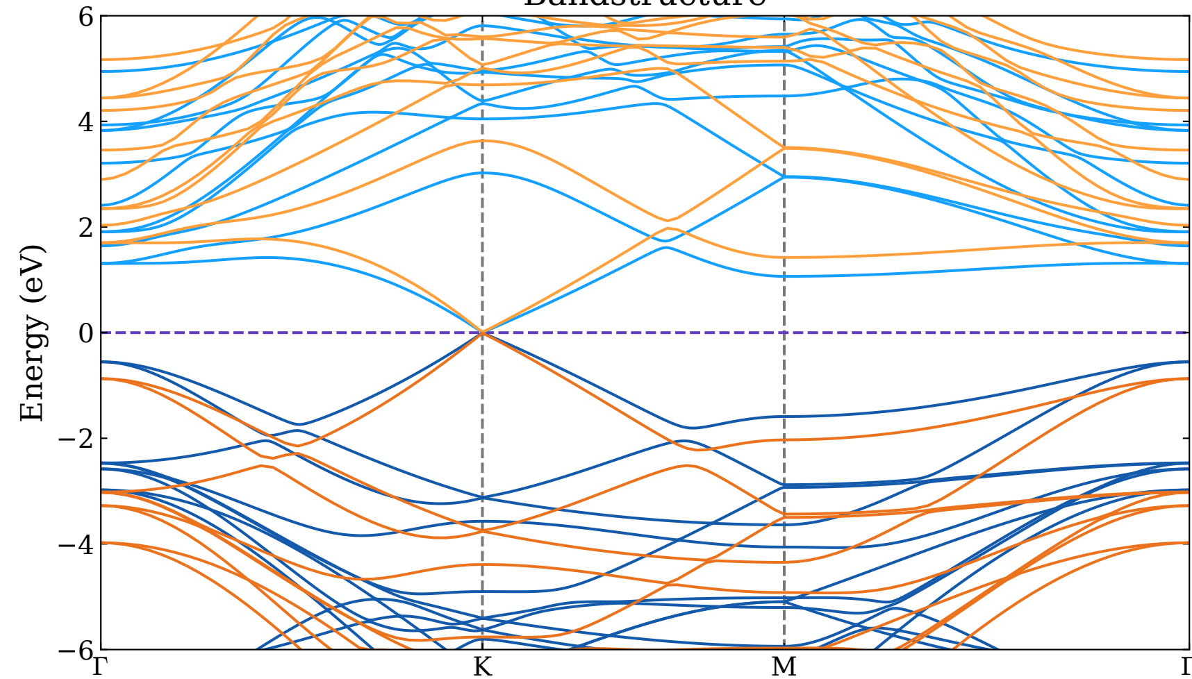
Bandstructure
